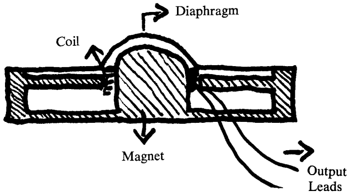
Figure 15. Dynamic Microphone.
