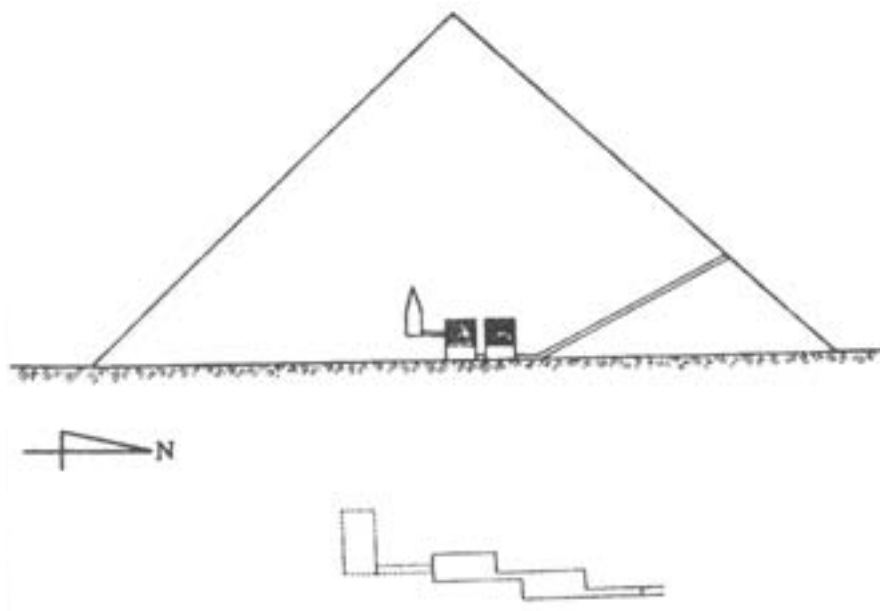
Figure 16.7: Section and plan of the Red Pyramid
