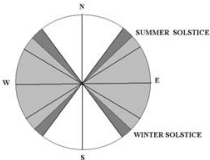
Figure A1.3: The rising-setting azimuths of the moon at the two standstills (heavy solid lines) compared with those of the sun.
