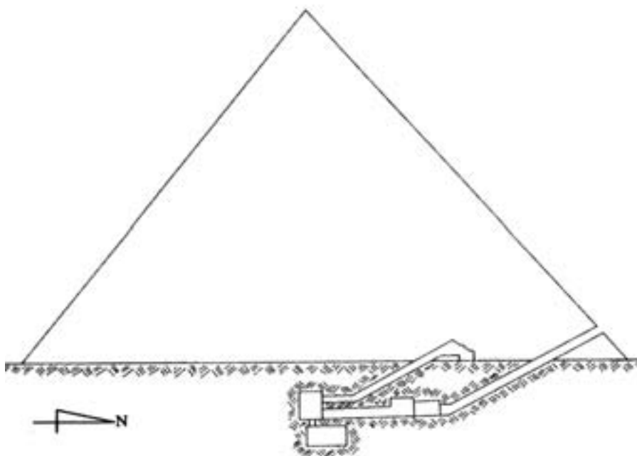
Figure 16.17: Section of Menkaure pyramid
