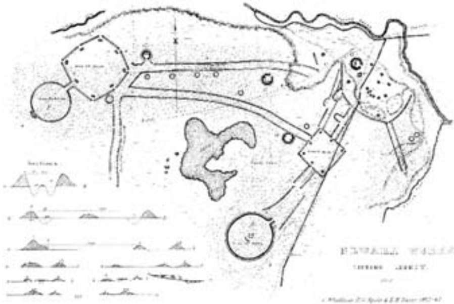
Figure 6.5: Newark earthworks
