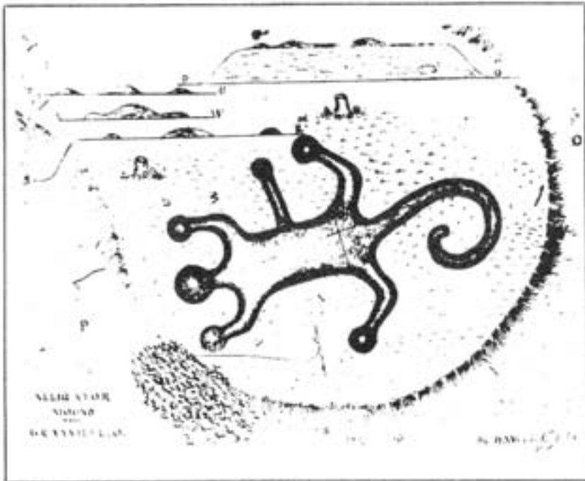
Figure 6.4: Alligator Mound
