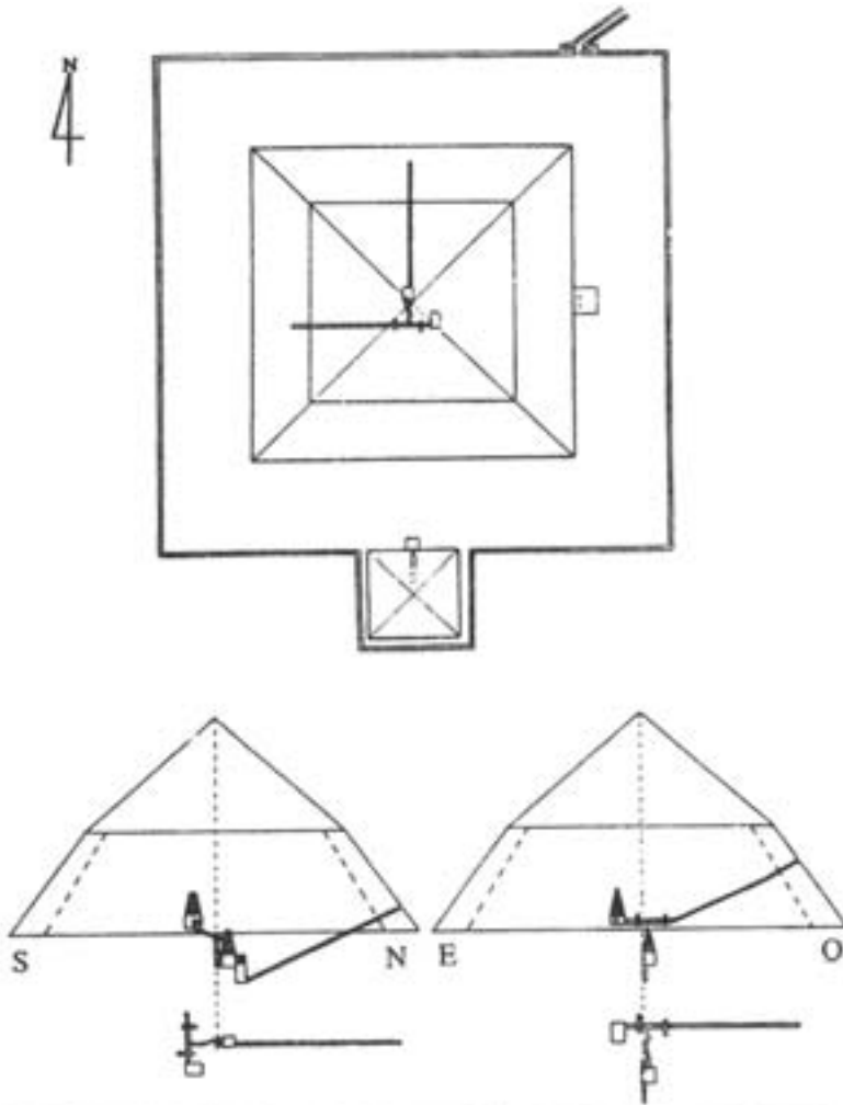
Figure 16.6: Plan, N-S and E-W sections of the Bent Pyramid.
