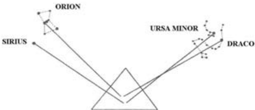
Figure 17.2: Astronomical alignments of the "air" shafts
