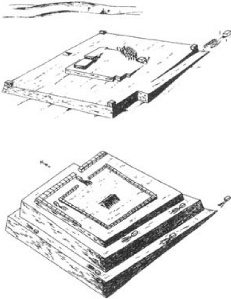
Figure 16.4: A reconstruction of the building site of the Great Pyramid (the dimensions of the blocks are exaggerate however).
