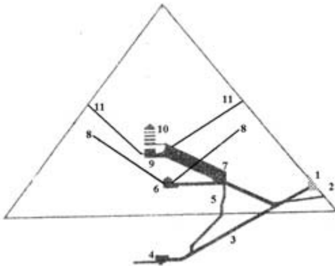
Figure 16.8: Section of the Great Pyramid. 1) Original entrance 2) Mamun's hole 3) Descending corridor 4) Subterranean Chamber 5) well shaft 6) Queen's Chamber 7) Great Gallery 8) Lower shafts 9) King's chamber 10) "Relieving Chambers" 11) Upper shafts
