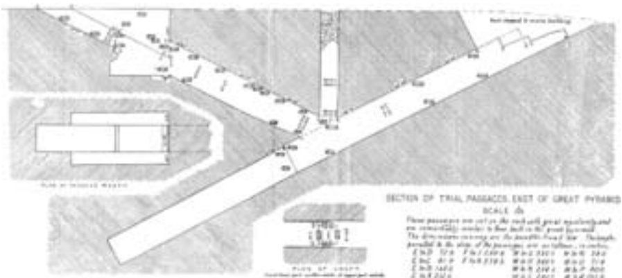
Figure 16.10: Section and plan of the "Trial Passages" according to Petrie
