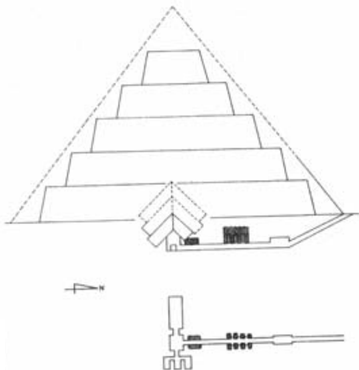
Figure 16.19: Section of the pyramid of Teti
