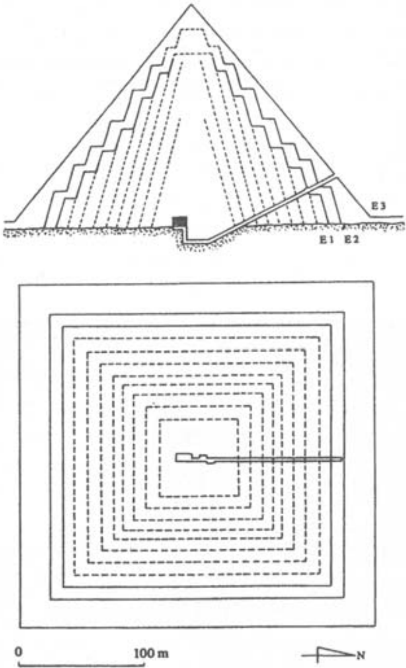
Figure 16.3: Section and plan of Meidum pyramid according to Burkhart
