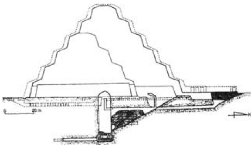
Figure 16:1: Section of the Djoser Step Pyramid, with the subsequent construction phases according to Lauer.
