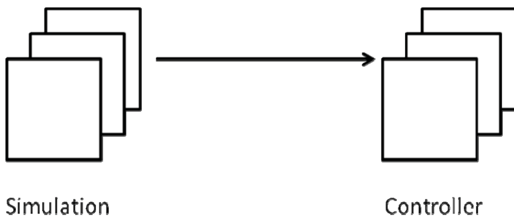
Figure 6.10 Pseudocode Transfer
