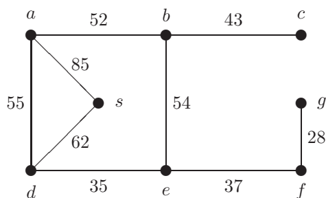
Figure 3.1: A Network with Costs
