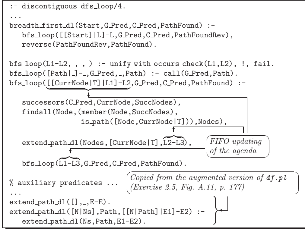
Figure A.14: Clauses Added to bf.pl
