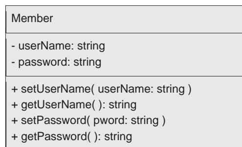
Figure 2.2 Simplified class diagram for the Member class
