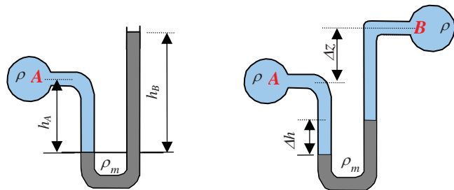
U-tube manometer
