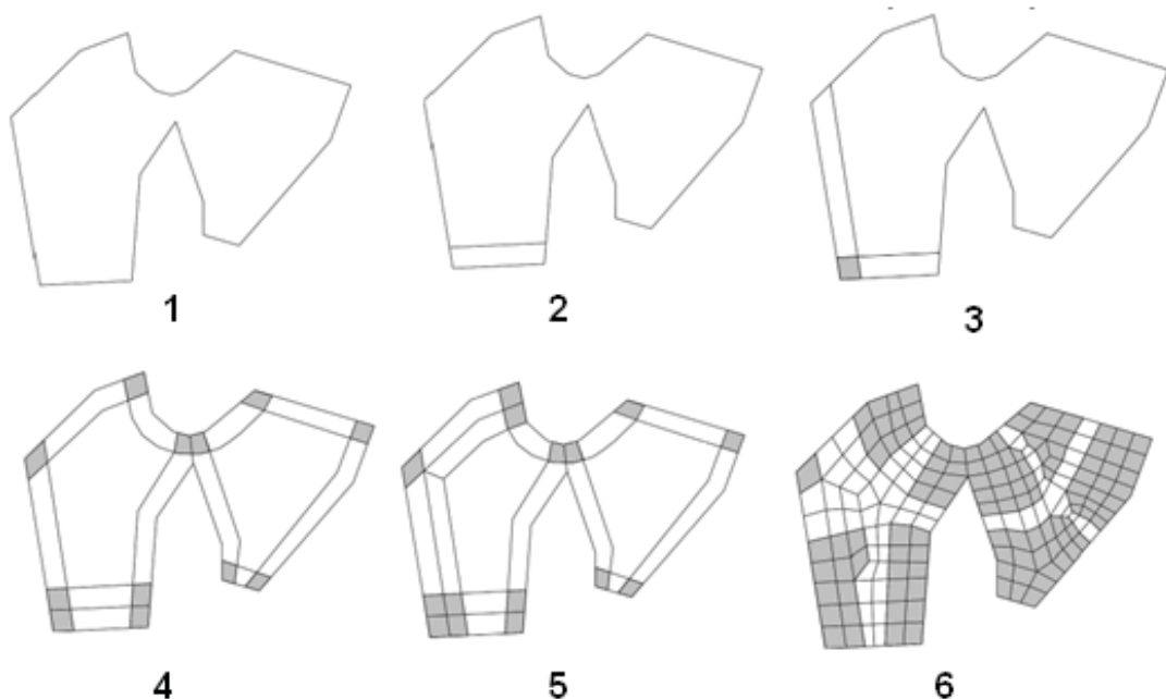
Figure 9.11 Paving
