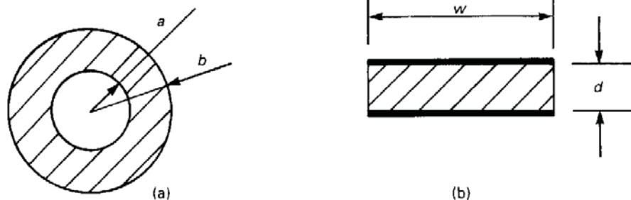
Fig. 6.11 (a) Coaxial and (b) parallel strip geometries
