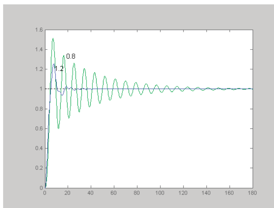
Figure 9.7 Step responses for closed loop with controller and plant for different natural frequencies of the plant poles.
