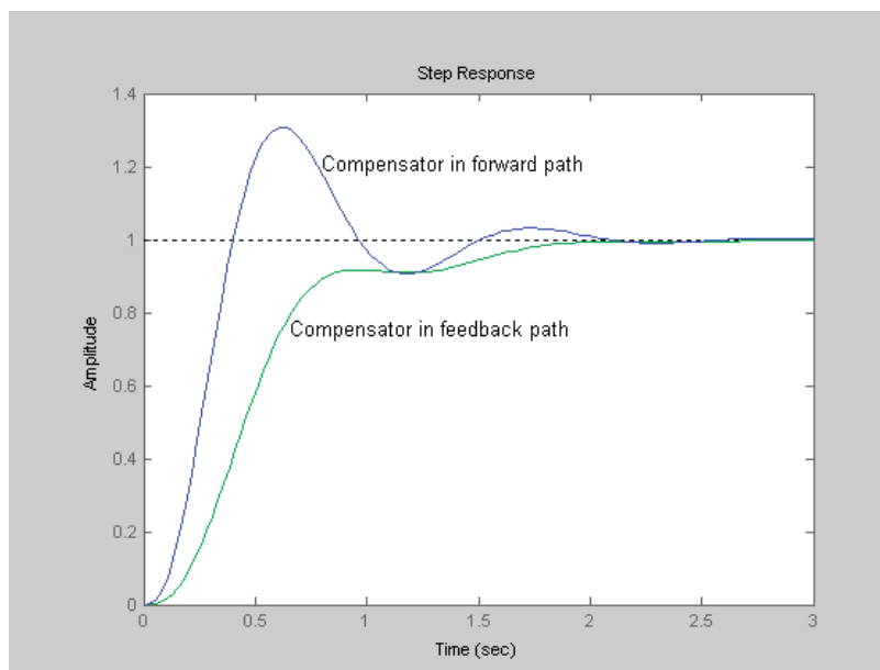
Figure 7.5 Comparison of step responses for forward path and feedback path locations of the compensator.
