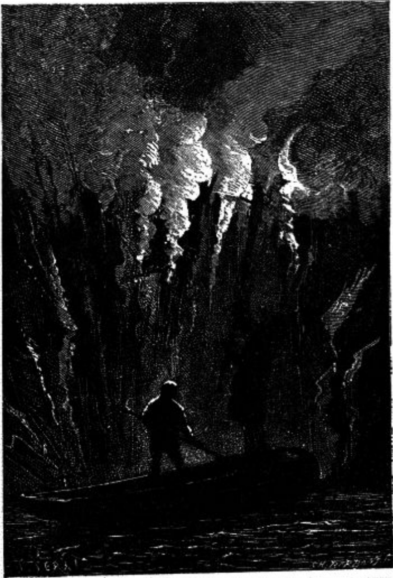
THE VOLCANO WALL IN DAKKAR GROTTA
