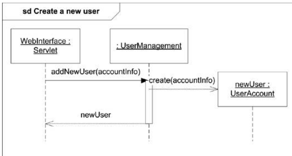
Figure 10-9. Object instantiation with the object lined up with the creation message
