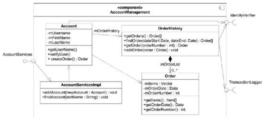
Figure 5-12. Component realization with ports and connectors
