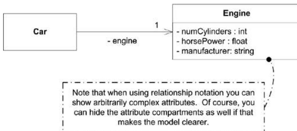
Figure 2-4. Attribute using relationship notation
