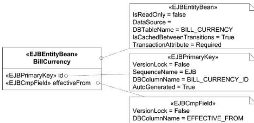
Figure 11-7. A stereotyped class and its stereotyped attributes, with their respective tagged values
