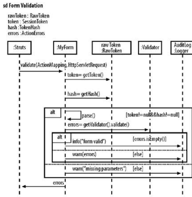
Figure 12-6. Sequence diagram with scope restricted to programmer-defined classes
