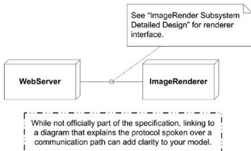
Figure 6-12. A communication path with a note attached
