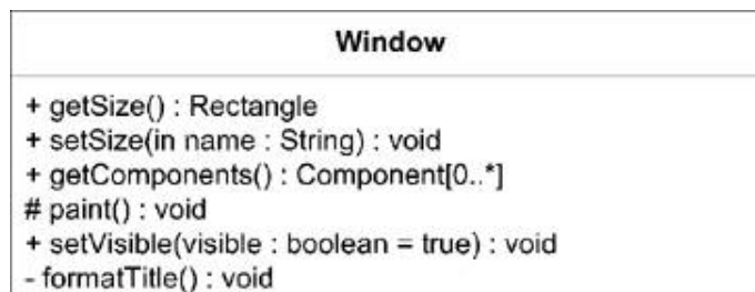
Figure 2-13. Example operations on a class
