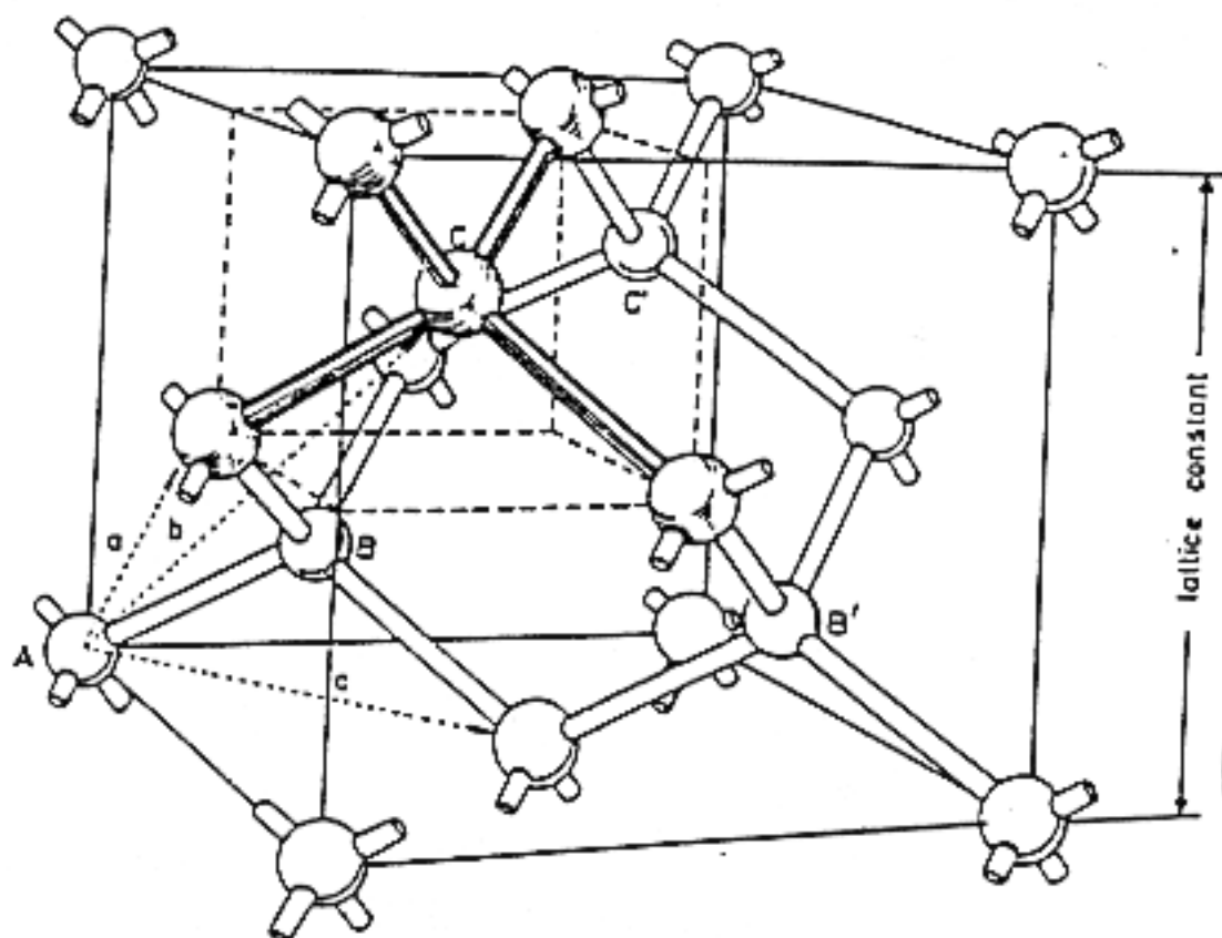
Diamond crystal structure. The lattice constants for C, Si, and Ge are 0.356, 0.543, and 0.566 nm, respectively.
