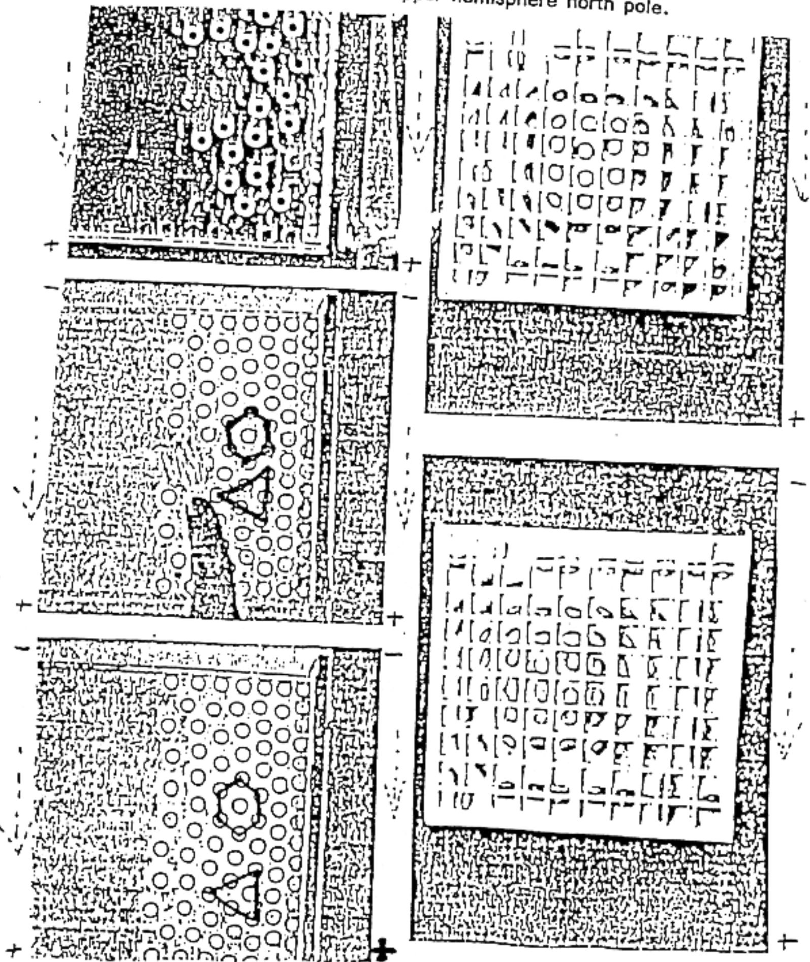
The expanding white hole lower hemisphere south pole.
