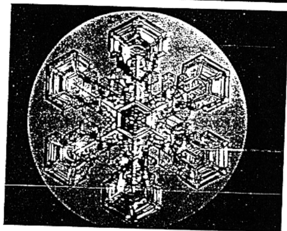
1. Photomicrographs of typical natural snow crystals, showing almost perfect hexagonal symmetry in their habit. The crystals are, in each case, approximately 2 mm in diameter (Magono & Lee, 1966).
