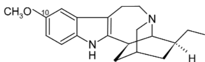
Ibogaine
