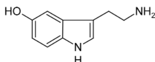
Serotonin
