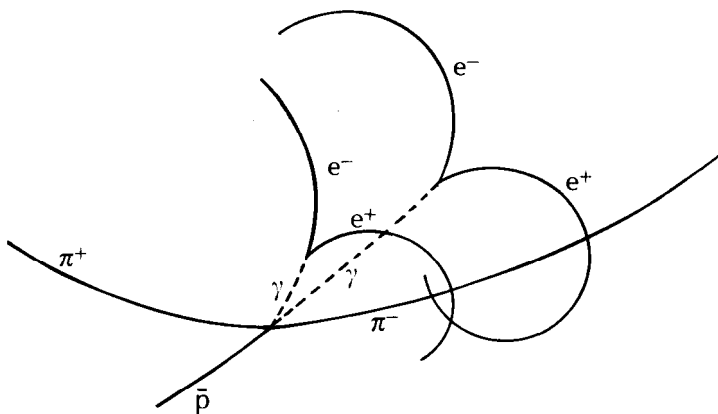
A sequence of events involving two pair creations: an antiproton ( \bar{p} ), coming in from below, collides with one of the protons in the bubble chamber to create a \pi^+ (flying off to the left), a \pi^- (flying off to the right), and two photons ( \gamma ), each of which creates an electron-positron pair, the positrons ( e^+ ) curving to the right, the electrons ( e^- ) to the left.
