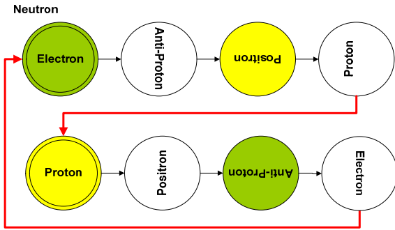
Figure 14. Neutron diagram
