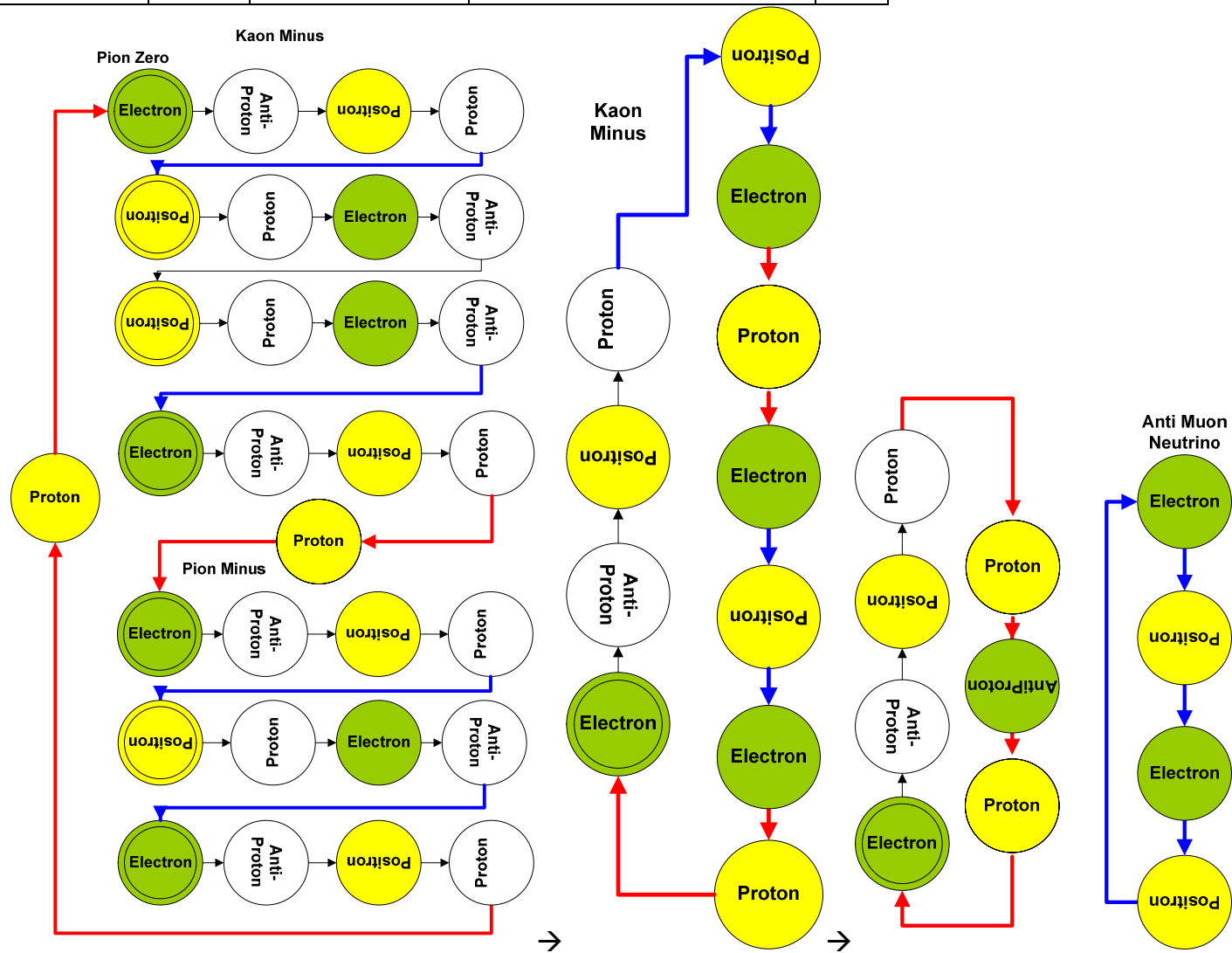
Figure 30. Kaon Minus decay diagram.
