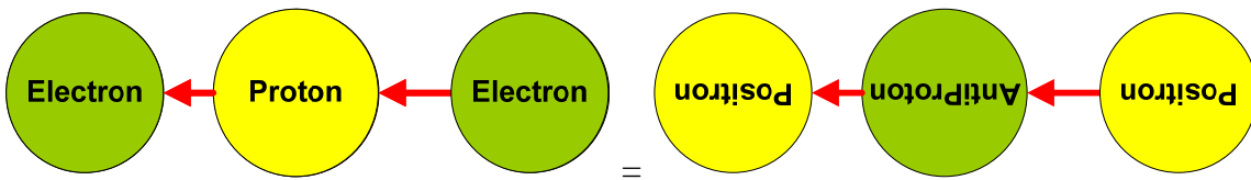
Figure 28. Delta Plus Plus decay diagram.
