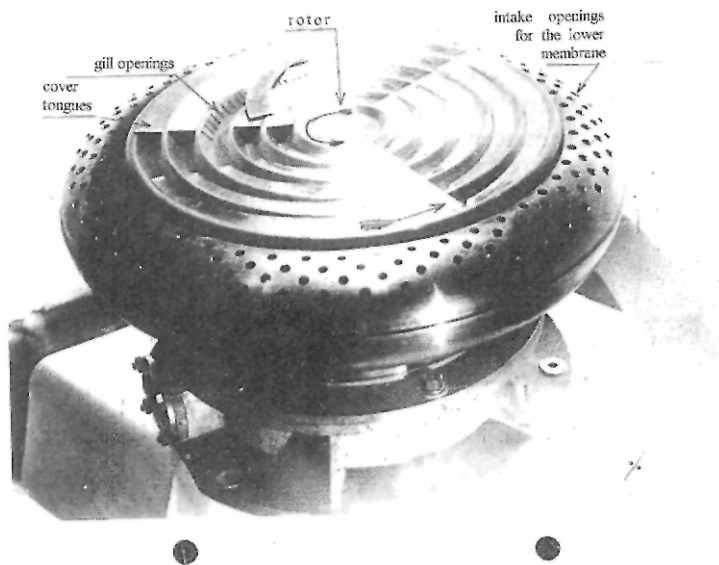
Fig. 31: Repulsine patent
