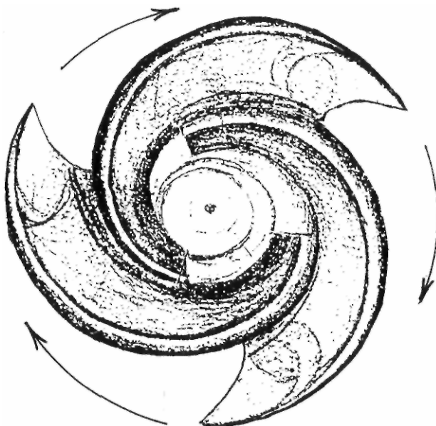
Fig. 11: 3-blade Bio-impeller
