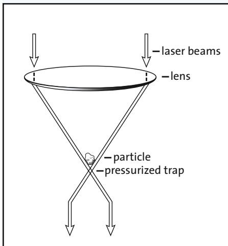
Illustration of dynamic optical tweezers (simplified).
