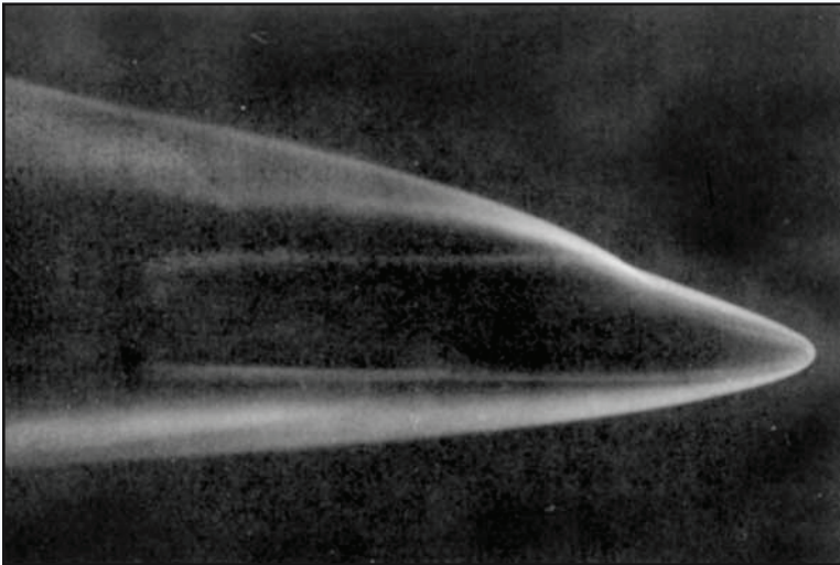
Graphic illustration of a supersonic wind-tunnel model during test, photographed by N+2 plasma light. (Courtesy of Hampton Roads Publishing)
