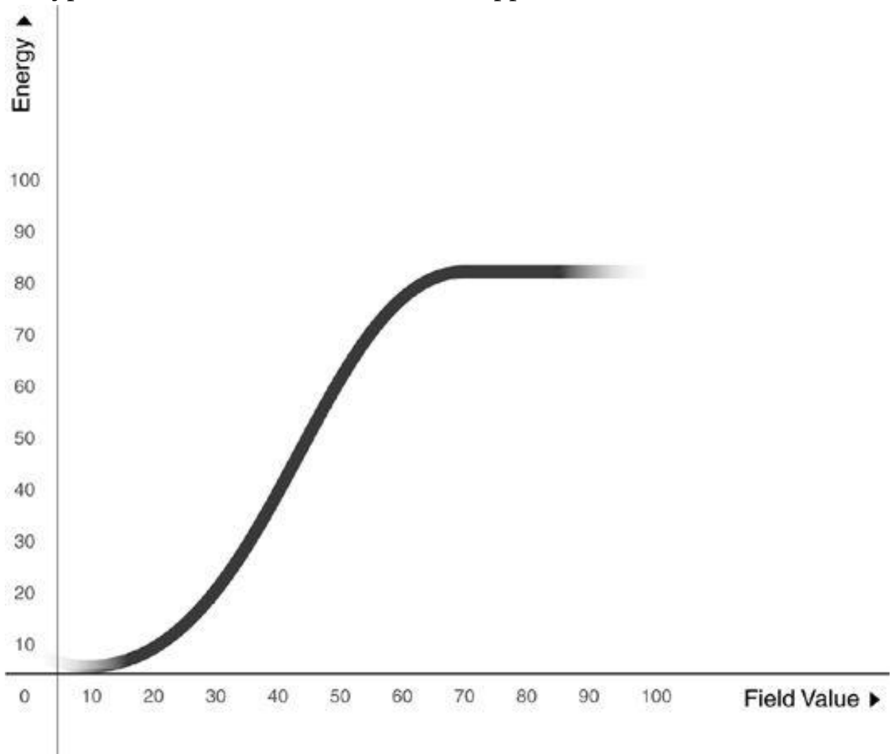
Figure 3.1 The energy contained in an inflaton field (vertical axis) for given values of the field (horizontal axis).
