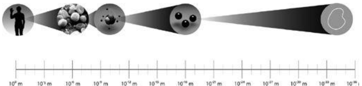
Figure 4.2 String theory's proposal for the nature of physics at the Planck scale envisions that the fundamental constituents of matter are string-like filaments. Because of the limited resolving power of our equipment, the strings appear as dots.
