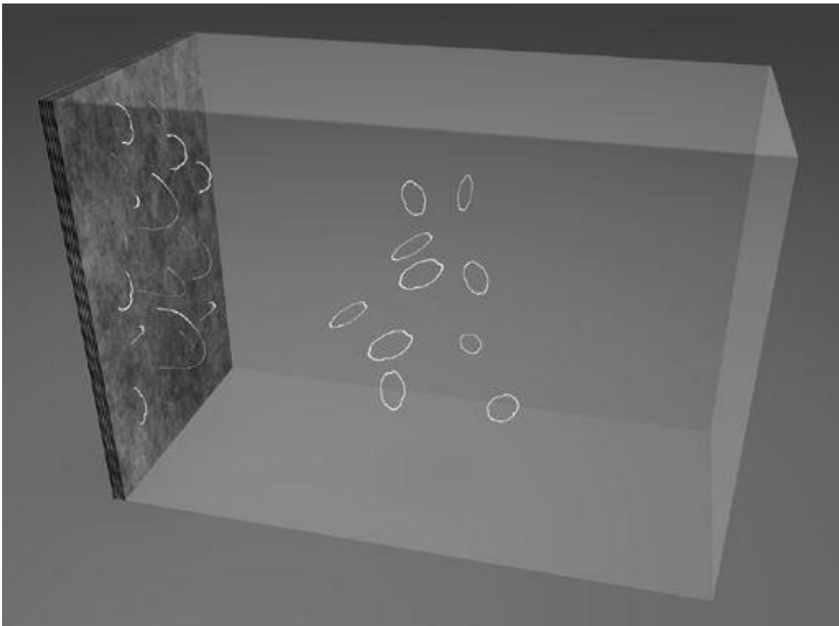
Figure 9.4 A collection of closely spaced three-branes with open strings confined to the brane surfaces, and closed strings moving through the “bulk.”
