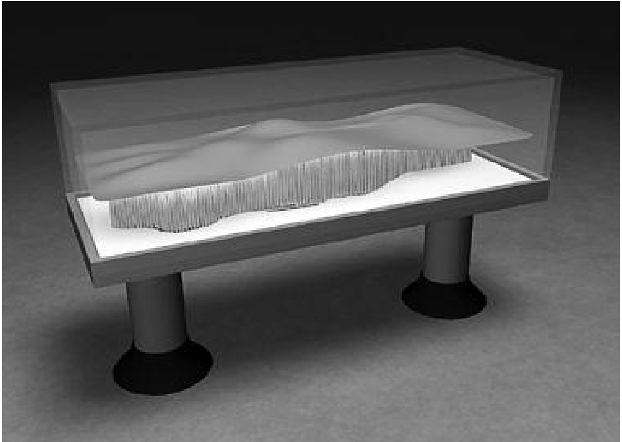
Figure 8.11 A general probability wave is the union of many spiked waves, each representing a possible position of the electron.
