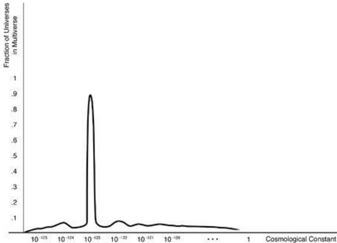
Figure 7.1 A possible distribution of cosmological constant values across a hypothetical multiverse, illustrating that highly skewed distributions can make otherwise puzzling observations understandable.
