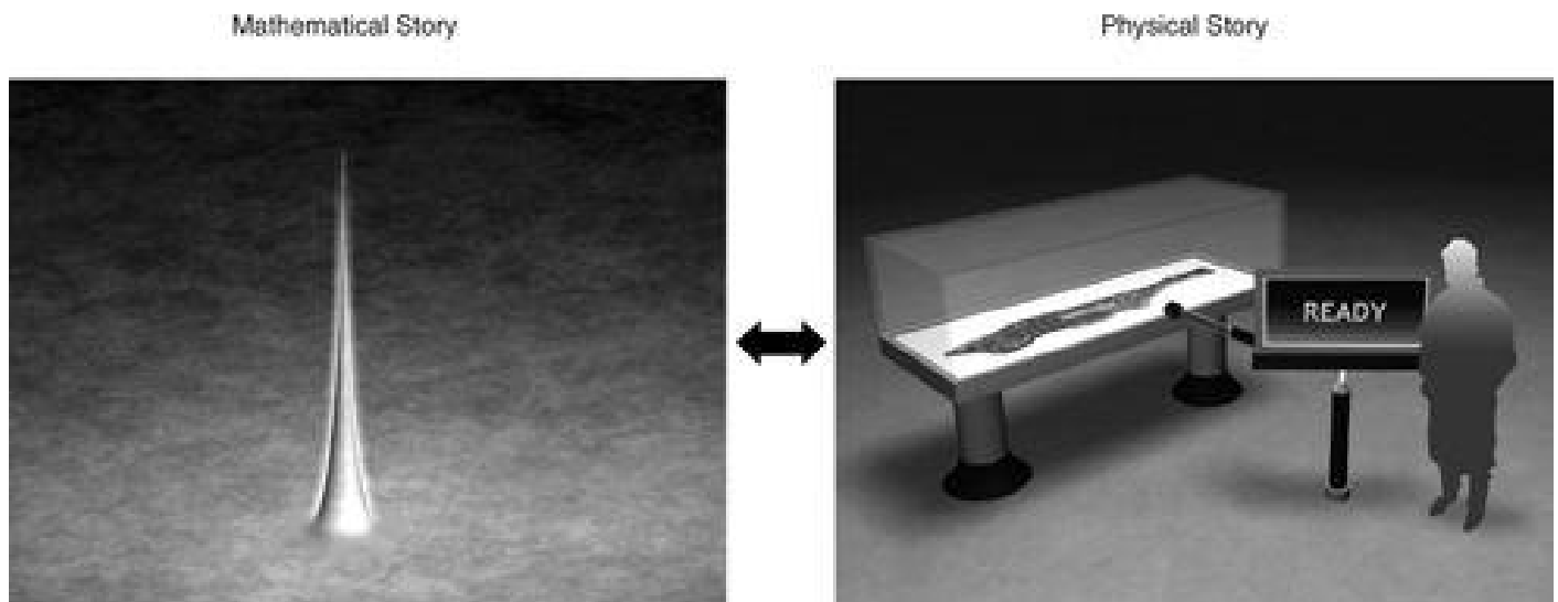
Figure 8.13 A schematic depiction of the combined probability wave for all the particles making up you and your measuring device.
