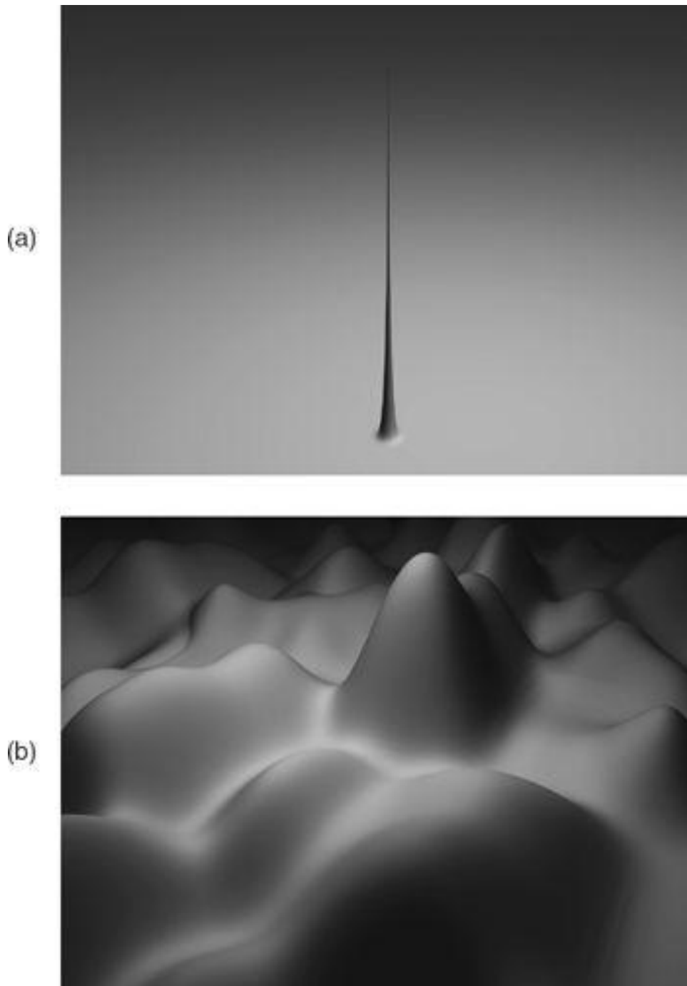
Figure 8.5 (a) The probability wave for a macroscopic object is generally narrowly peaked. (b) The probability wave for a microscopic object, say, a single particle, is typically widely spread.
