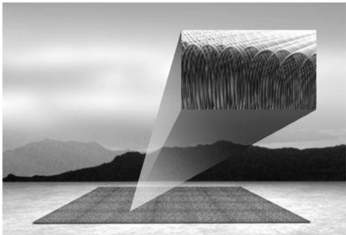
Figure 4.4 (a) The surface of a tall straw has two dimensions; the vertical dimension is long and easy to see, while the circular dimension is small and harder to detect. (b) A gigantic carpet has three dimensions; the north/south and east/west dimensions are big and easy to see, while the circular part, the carpet's pile, is small and therefore harder to detect.
