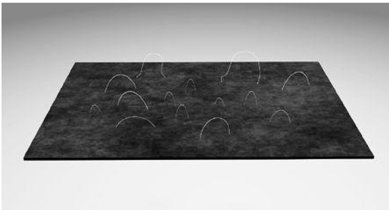
Figure 5.4 Branes are the only locations where the endpoints of string snippets can reside.
