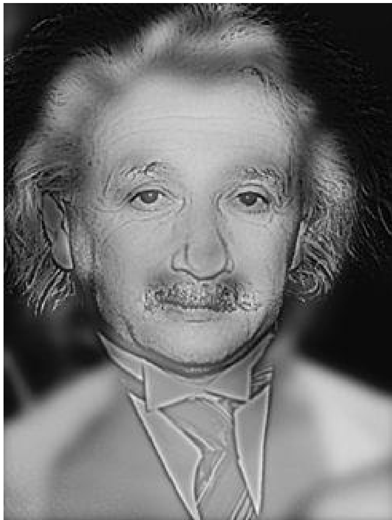
Figure 5.2 From close up, the image looks like Albert Einstein. From farther away, it looks like Marilyn Monroe. (The image was created by Aude Oliva of the Massachusetts Institute of Technology.)
