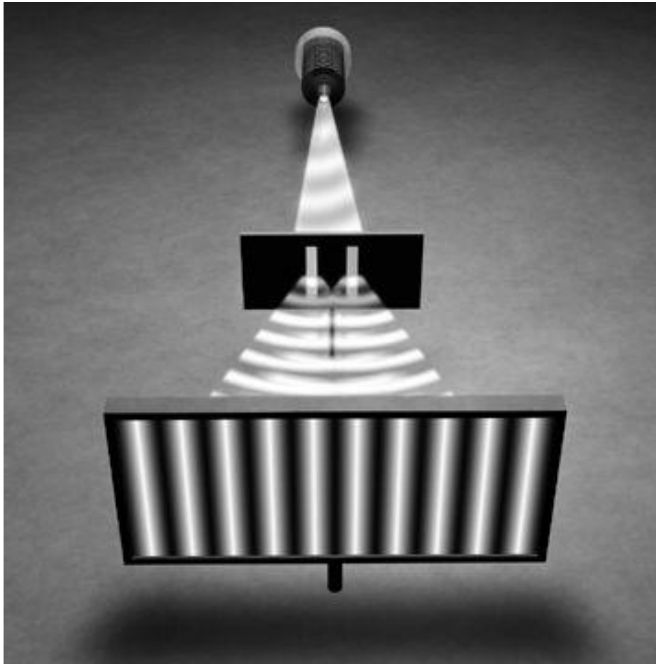
Figure 8.4 When we describe the motion of an electron in terms of an undulating probability wave, the puzzling interference data are explained.
