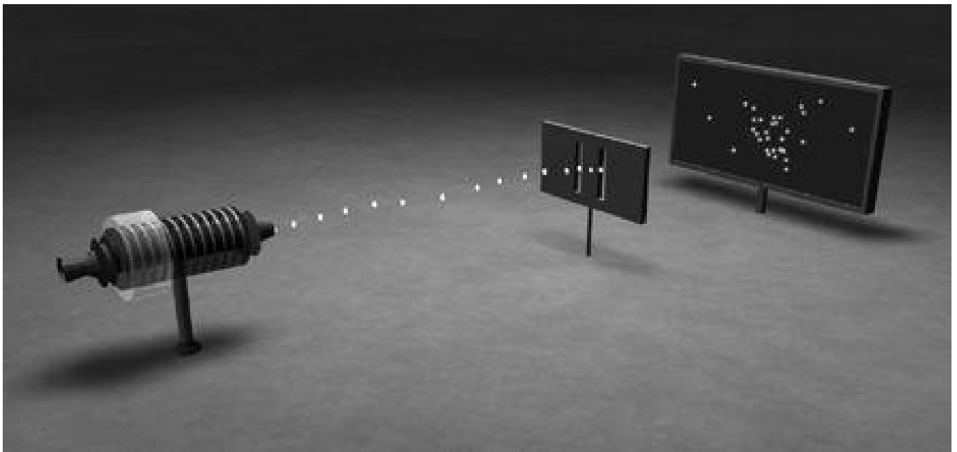
Figure 8.1 The essence of the Davisson and Germer experiment is captured by the “double-slit” setup in which electrons are fired at a barrier that has two narrow slits. In the Davisson and Germer experiment, two streams of electrons are produced when incident electrons bounce off neighboring nickel crystals; in the double-slit experiment, two similar streams are produced by electrons that pass through the neighboring slits.
