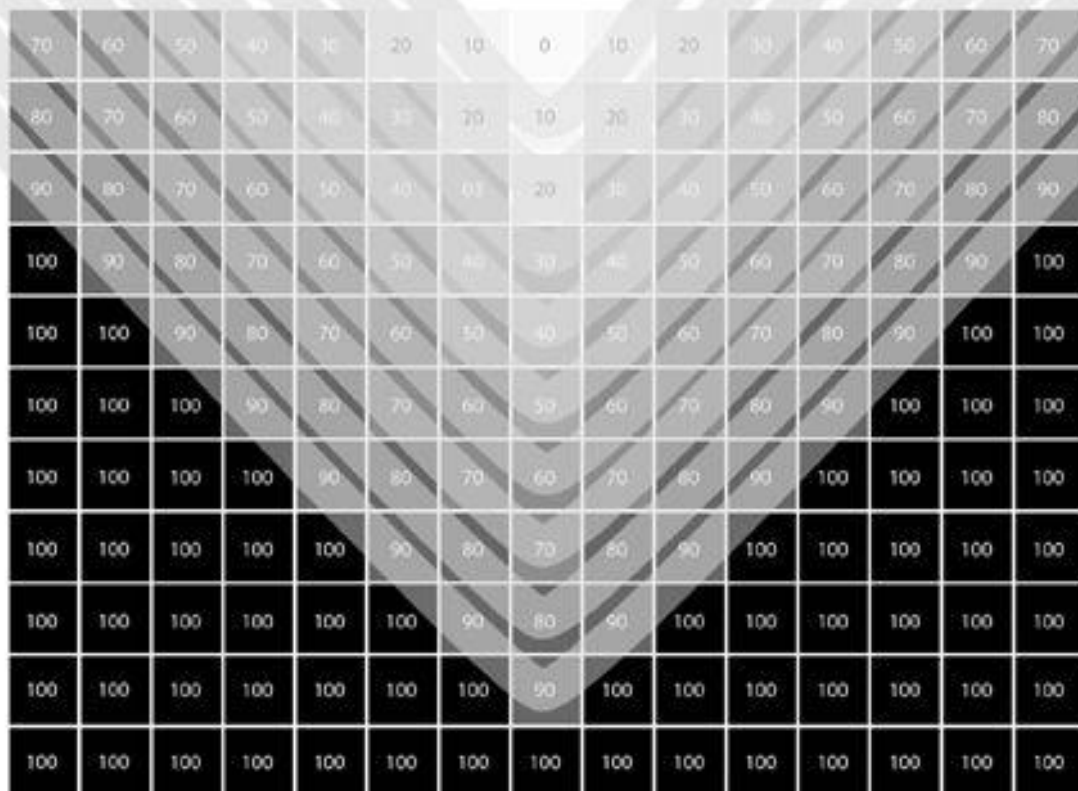
Figure 3.8b The same information as in Figure 3.8a is organized differently by someone within the bubble. Inflaton values that agree correspond to identical moments, so the curves drawn sweep through all those points in space that exist at the same moment in time. Smaller inflaton values correspond to later moments. Note that the curves could be extended infinitely far, so from an insider's perspective, space is infinite.
