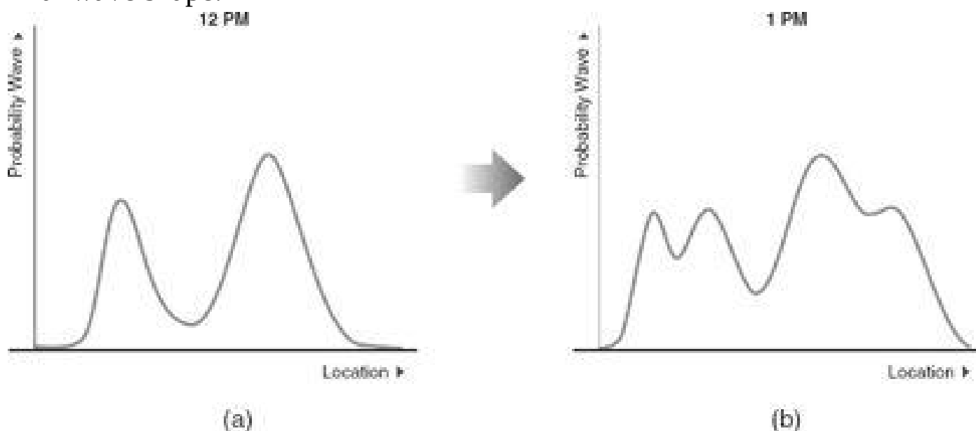
Figure 8.7 (a)An initial probability wave shape at one moment evolves via Schrödinger's equation to a different shape(b)at a later time.
