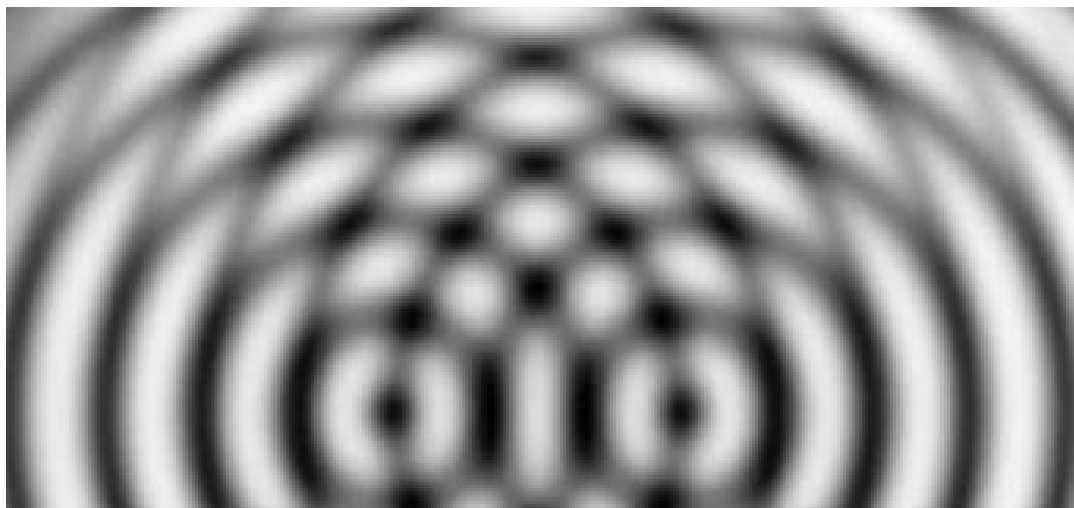
Figure 8.3 When two water waves overlap, they “interfere,” creating alternating regions of more or less agitation called an interference pattern.
