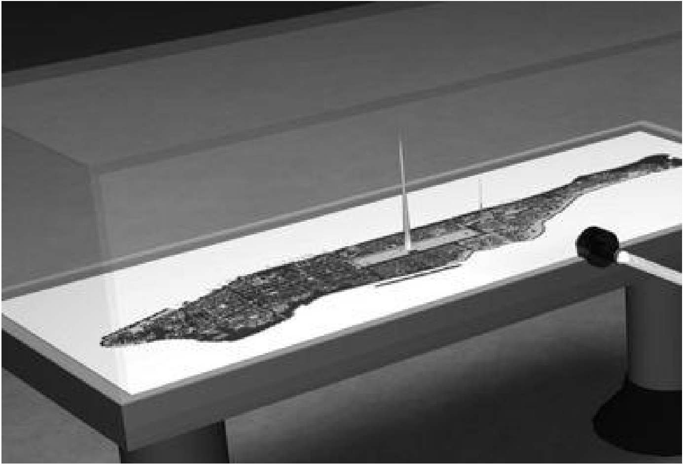
Figure 8.17 The combined probability wave for you and your device encounters a probability wave that has multiple spikes of different magnitudes.
