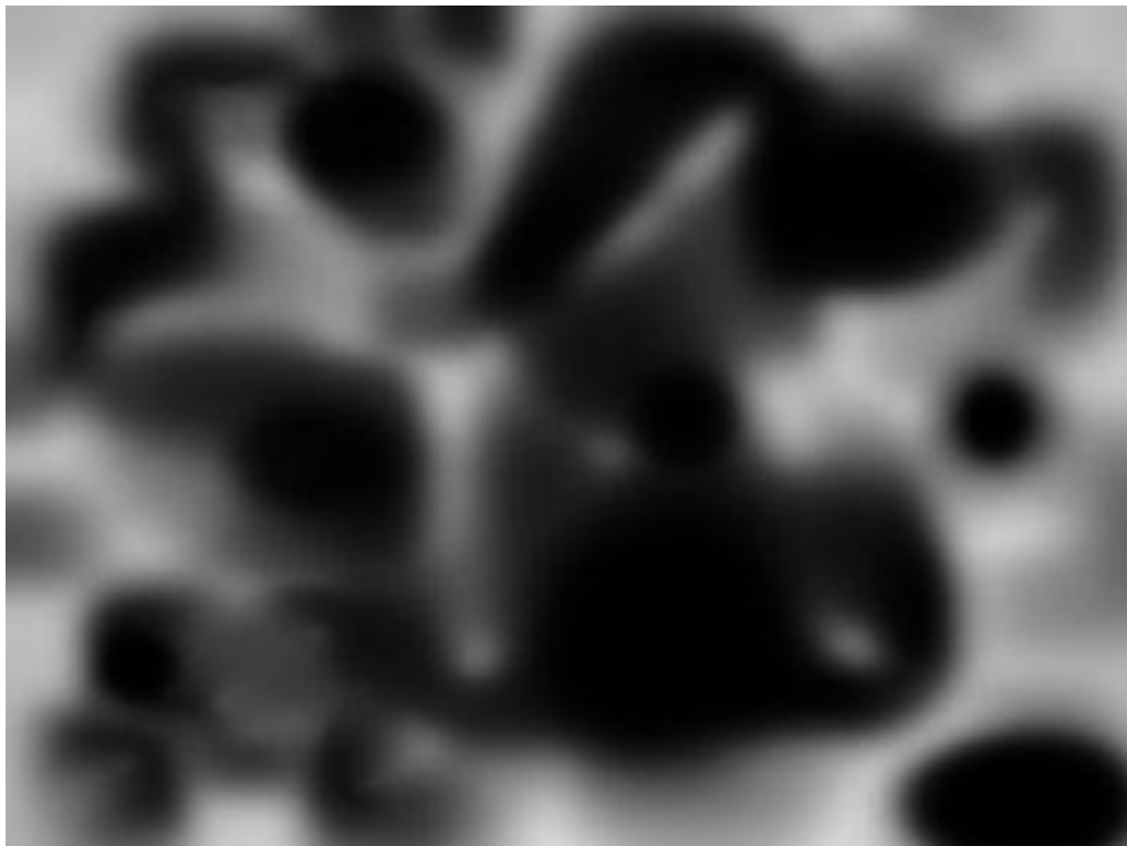
Figure 3.2 Various domains in which the inflaton field has dropped down the slope (darker gray) or remains high (lighter gray).
