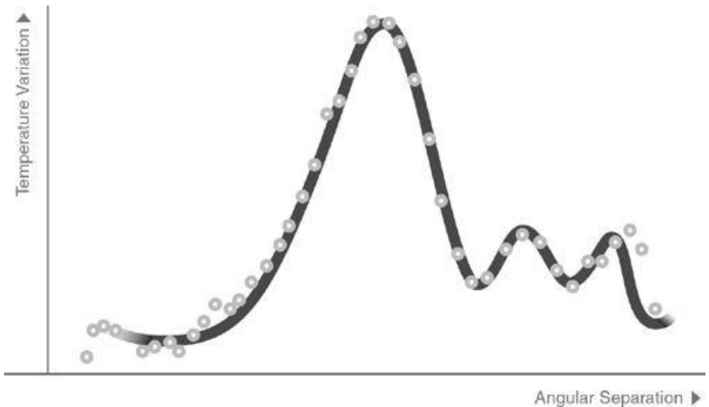
Figure 3.5 The pattern of temperature differences in the cosmic microwave background radiation. Temperature variation is the vertical axis; the separation between two locations (measured by the angle between their respective lines of sight when viewed from earth—larger angles to the left, smaller angles to the right) is the horizontal axis. 11 The theoretical curve is solid; the observational data are given by the circles.
