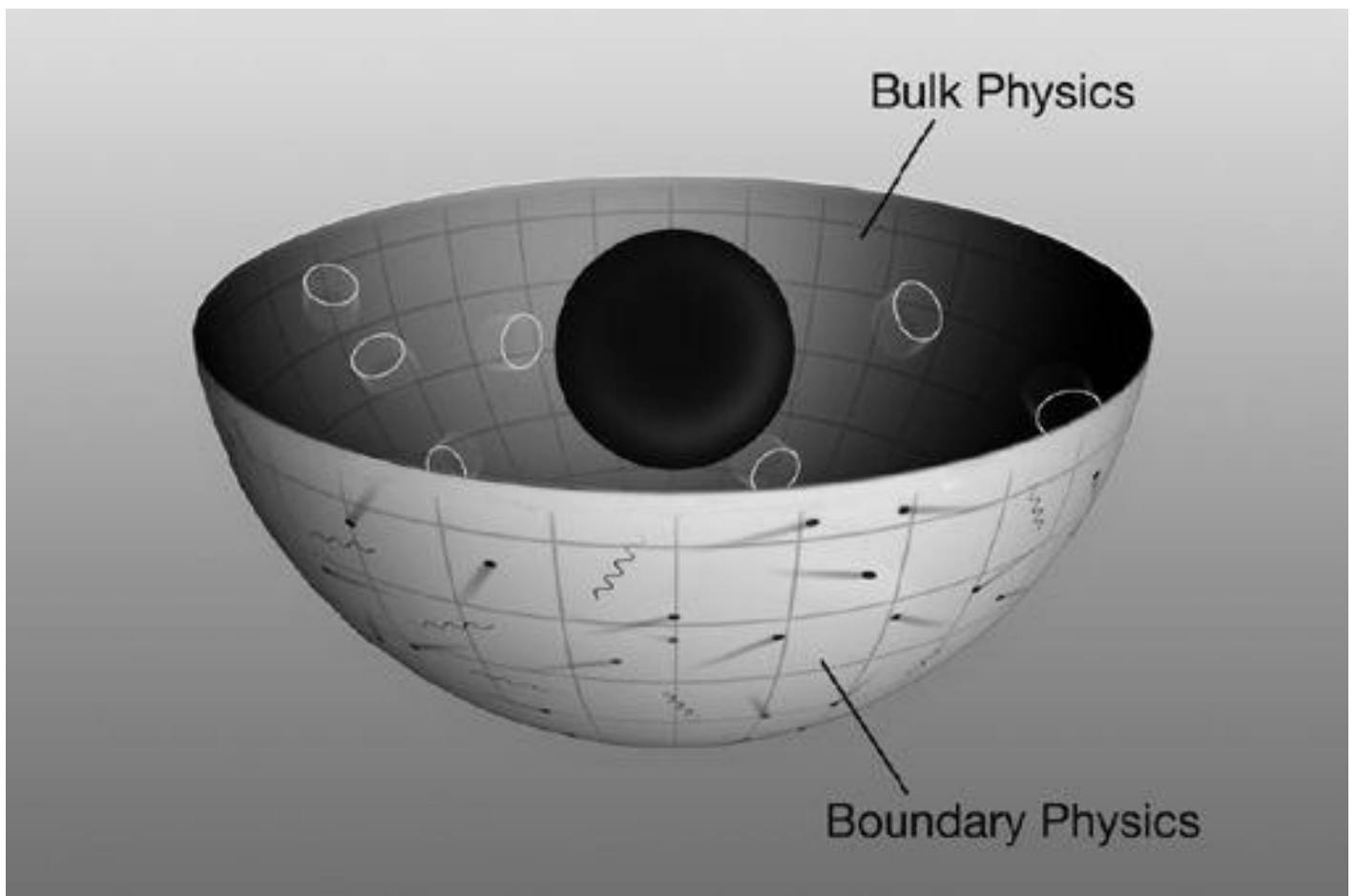
Figure 9.6 The holographic equivalence applied to a black hole in the bulk of spacetime yields a hot bath of particles and radiation on the region's boundary.
