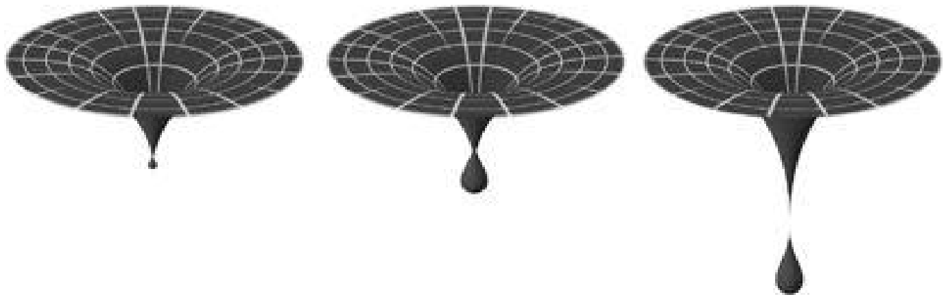
Figure 10.1 Because of the greater pressure in the ambient environment, an inflationary seed is forced to expand into newly formed space. As the bubble universe grows, it detaches from the parent environment, yielding a separate, expanding spatial domain. To someone in the ambient environment, the process looks like the formation of a black hole.
