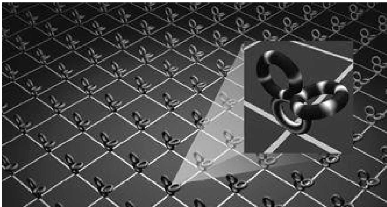
Figure 5.6 Parts of the extra dimensions in string theory can be wrapped by branes and threaded by fluxes, yielding “dressed-up” Calabi-Yau shapes. (The figure uses a simplified version of a Calabi-Yau shape—a “three-hole doughnut”—and represents wrapped branes and flux lines schematically with glowing bands encircling portions of the space.)
