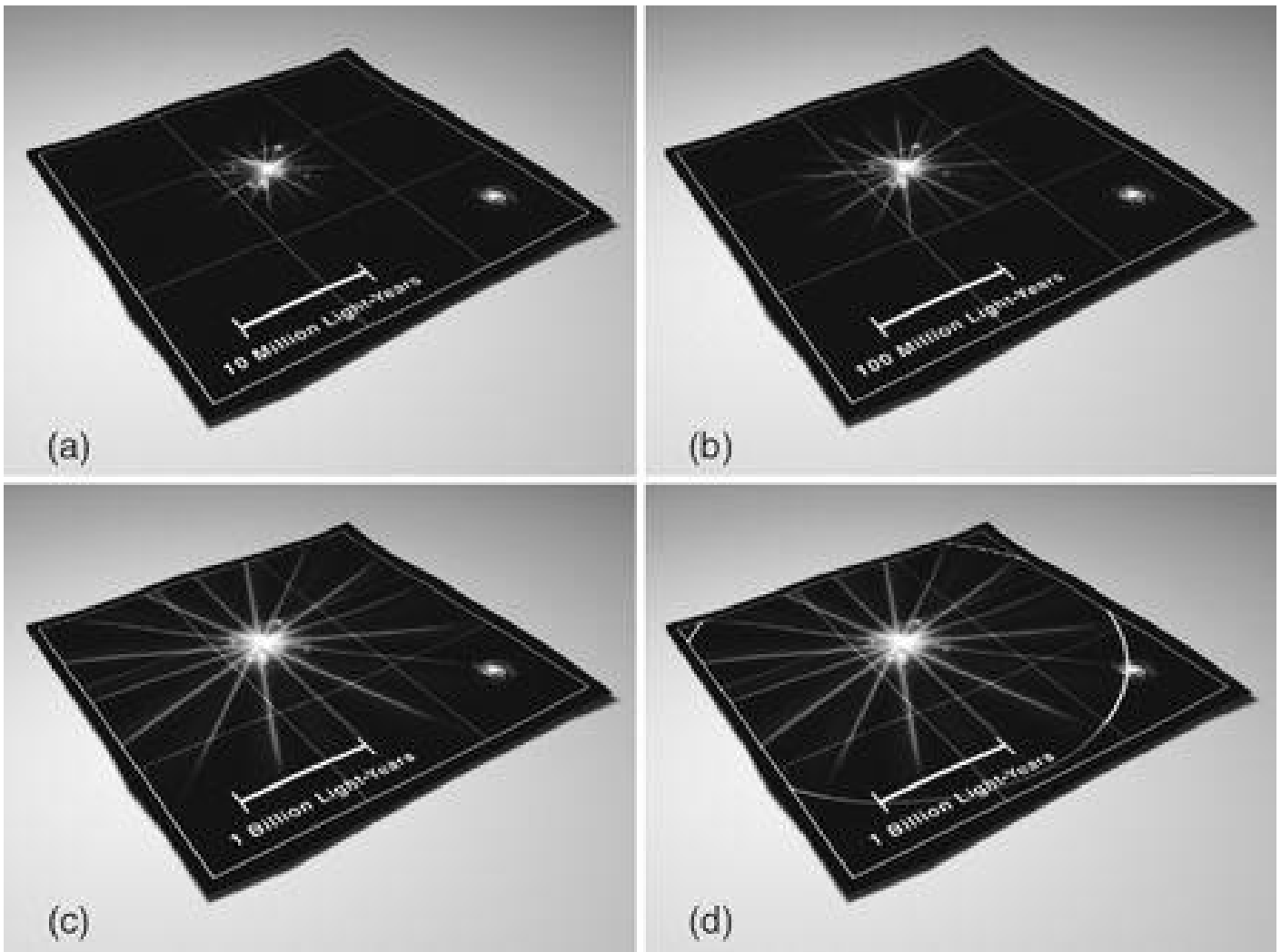
Figure 6.1 (a) Light from a distant supernova spreads as it travels toward us (we are situated in the galaxy on the map's right-hand side). (b) During the light's journey, the universe expands, which is reflected in the map's legend. (c) When we receive the light, its intensity has been diluted through the spreading. (d) When we compare the supernova's apparent brightness to its intrinsic brightness, we are measuring the area of the sphere on which it has spread (drawn as a circle), and hence also its radius. The radius of the sphere traces the light's trajectory. Its length is the distance now between us and the galaxy that contained the supernova, so that's what the observations determine.
