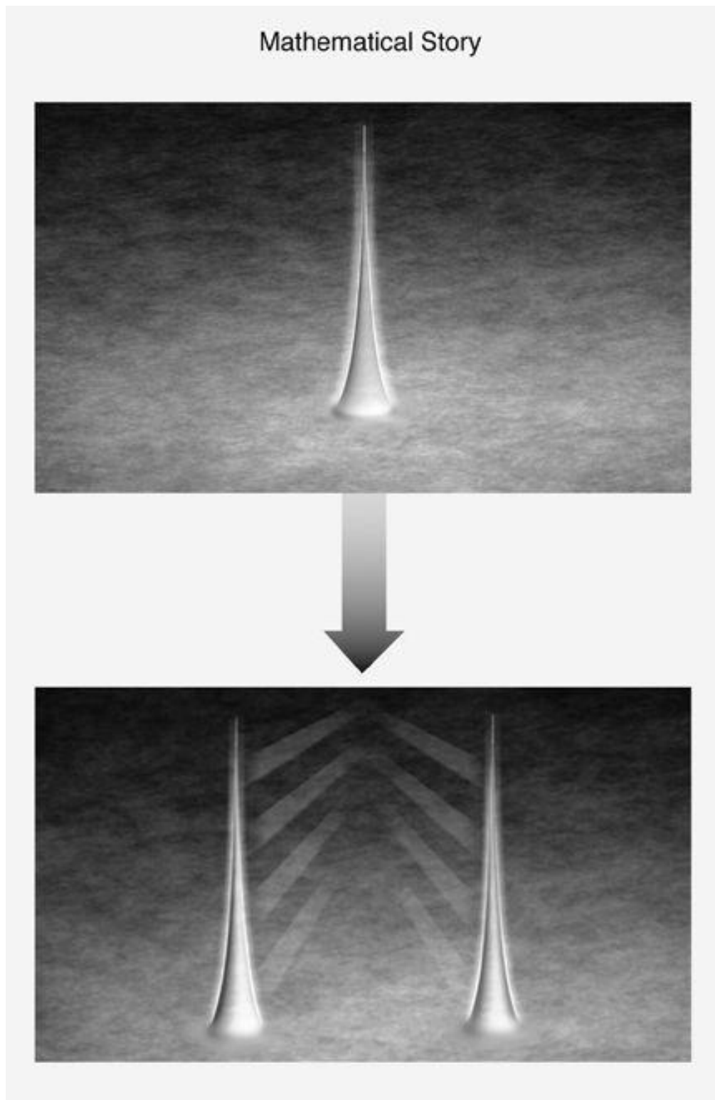
Figure 8.16 (a) A schematic illustration of the evolution of the combined probability wave of all the particles making up you and your device, when measuring the position of an electron whose probability wave is spiked at two locations.
