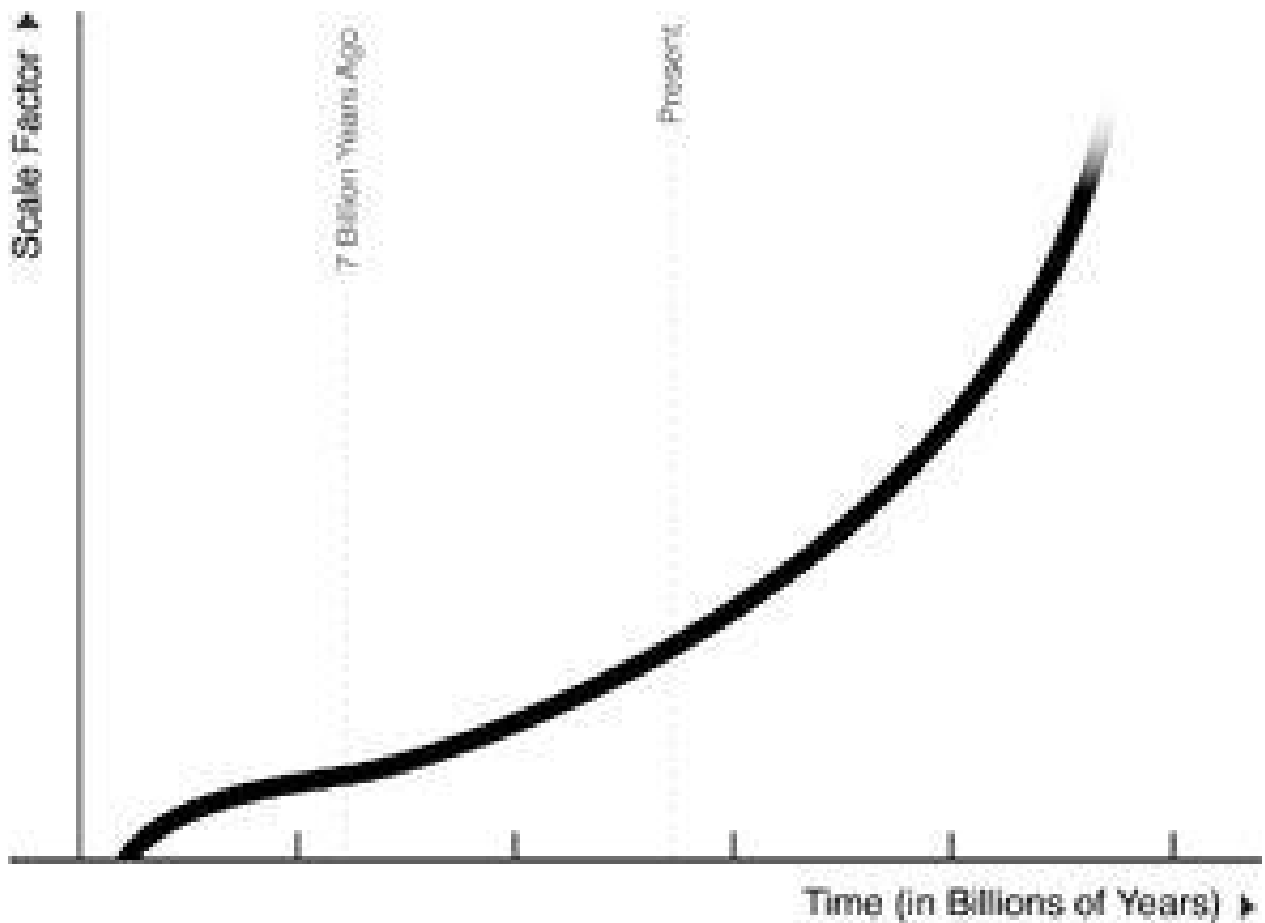
Figure 6.2 The scale factor of the universe over time, showing that cosmic expansion slowed down until about 7 billion years ago, when it began to speed up.
