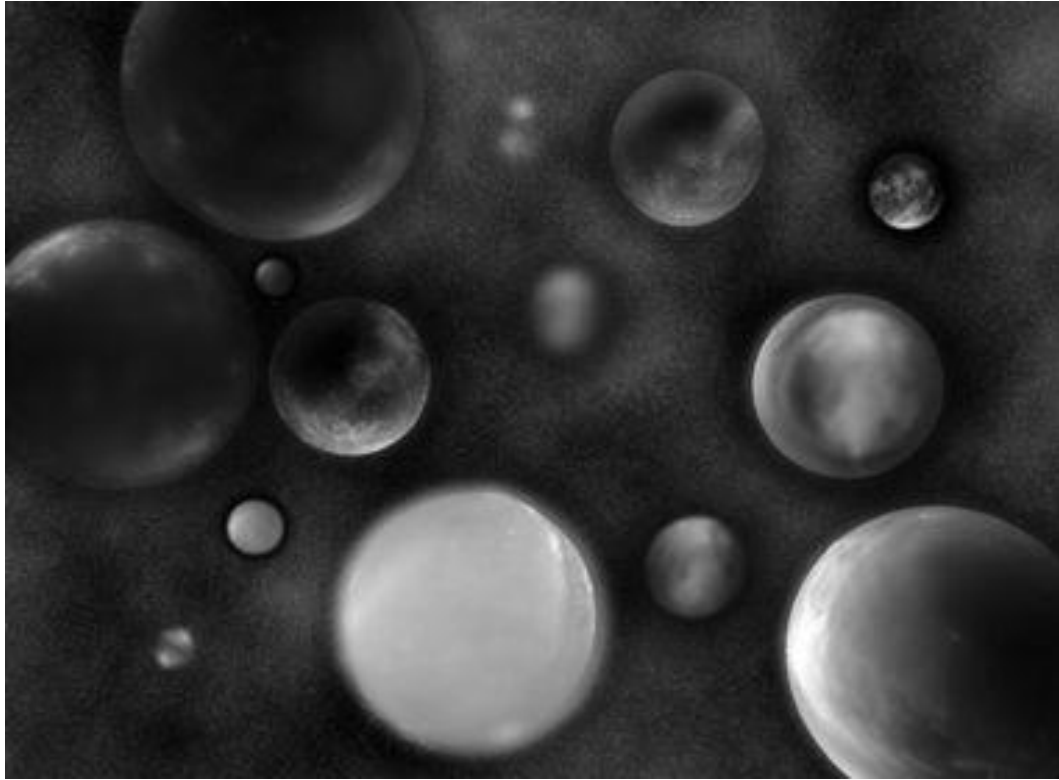
Figure 3.3 The Inflationary Multiverse arises when bubble universes continually form within an ever-expanding spatial environment permeated by a high-valued inflaton field.
