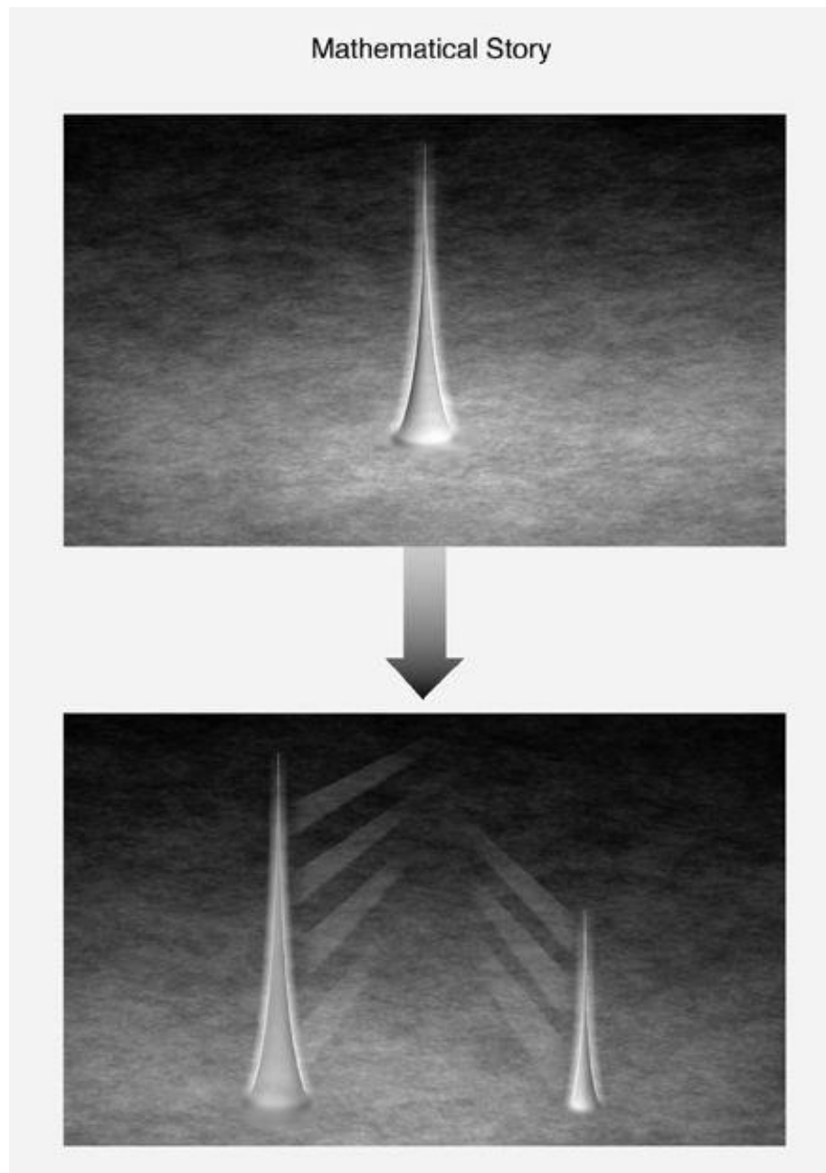
Figure 8.18 (a) A schematic illustration of the evolution, dictated by Schrödinger's equation, of the combined probability wave for all the particles making up you and the measuring device, when you measure the position of an electron. The electron's own probability wave is spiked at two locations, but with unequal wave heights.
