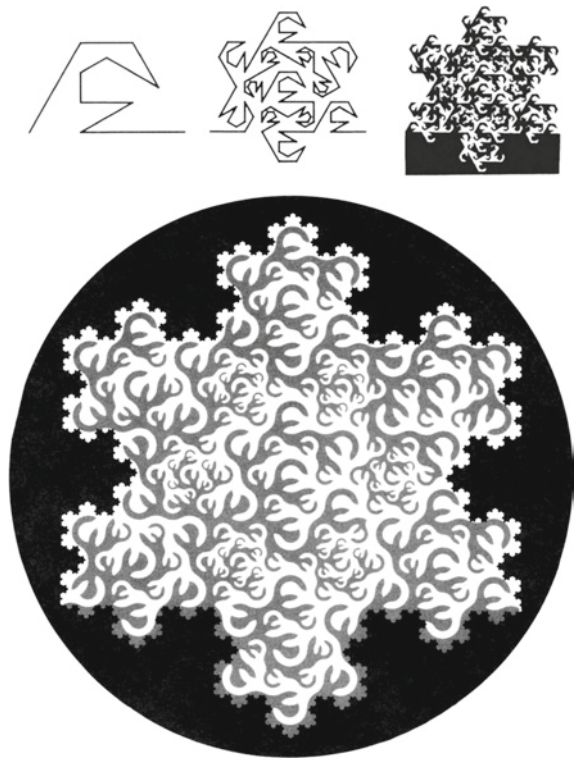
Fig. 3.7 above: Mandelbrot's Peano curve (B.B.Mandelbrot).
