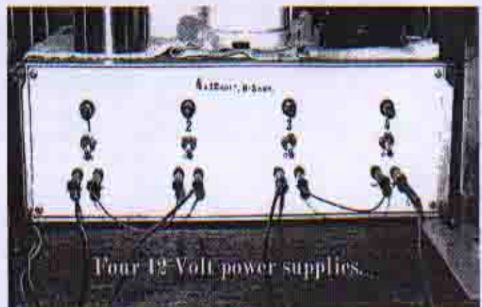
FIG 39. Power supply designed to separately charge 4 cells at one time. Alternatively the unit can be connected to supply 24 volts, 36 volts and 48 volts if required.
