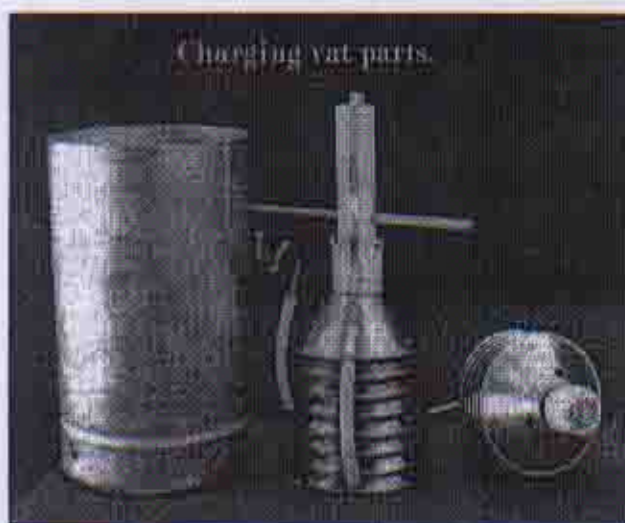
FIG 5. Charging Vat. Overall view of main components. I have shown two different types of cone stacks. The stack nearest to the Vat is the one used in this manual.
