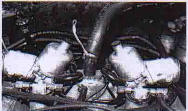
FIG 47. Engine to cell tube connection. Notice NO WORM CLIP on the plug ( engine ) end of the coupling hose. Short section of electrical wiring is connected to 'ignition - on ' positive wiring of the car as per text.
