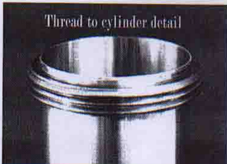
FIG 19. Cell - 5 cylinder. A view of the press fitted thread. Notice the position. The outer cylinder must be a metal to metal fit with the base cap
