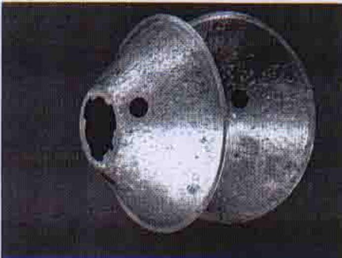
FIG 4. Cones from charging vat. This is the result of using over 10 Amps for long periods. Note the severe pitting. These cones are now junk.
