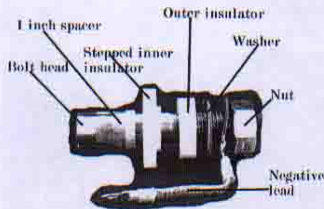
FIG 21. Cell - 5 cylinder. The correct cylinder assembly of the central cylinder bolt components
