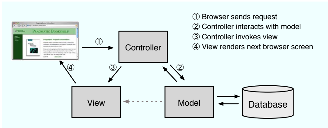
Figure 2.1: The Model-View-Controller Architecture
