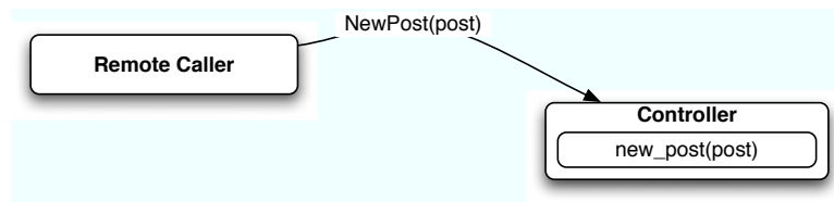
Figure 25.2: Overview of Direct Dispatching
