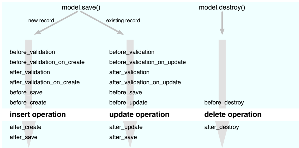
Figure 19.1: Sequence of Active Record Callbacks
