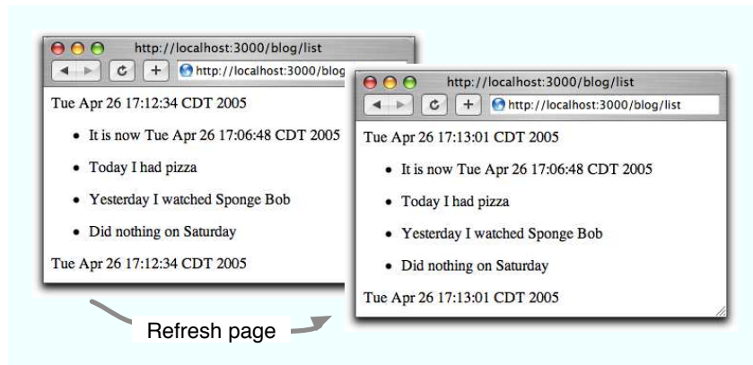
Figure 22.4: Refreshing a Page with Cached and Noncached Data
