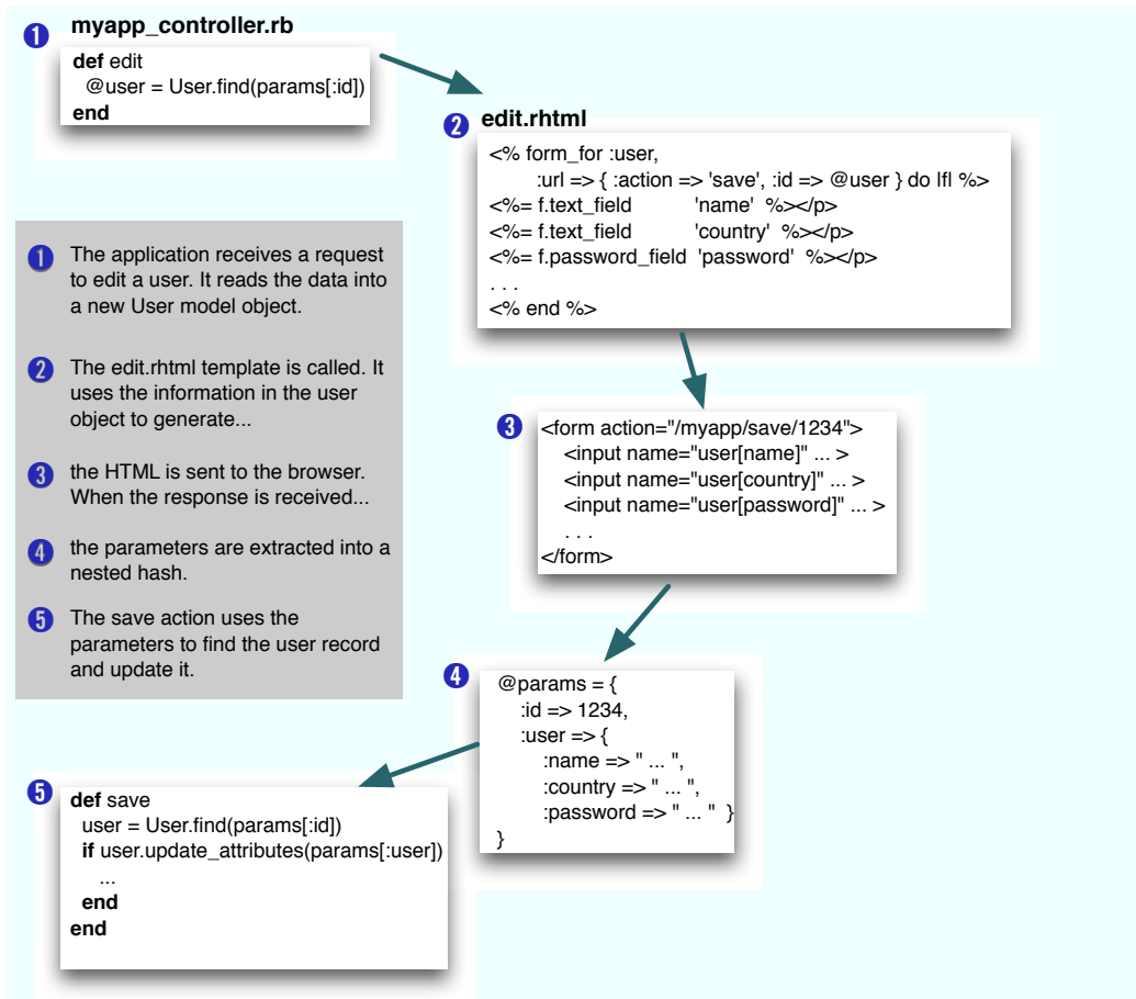
Figure 22.1: Models, Controllers, and Views Work Together
