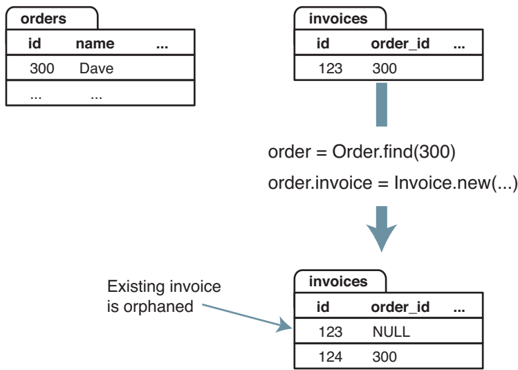
Figure 18.1: Adding to a has_one Relationship
