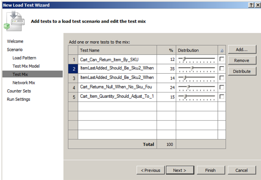
FIGURE 8-19: Next, you choose the tests (unit, Web, or other) and the percentage of load to create from each of the specific tests.
