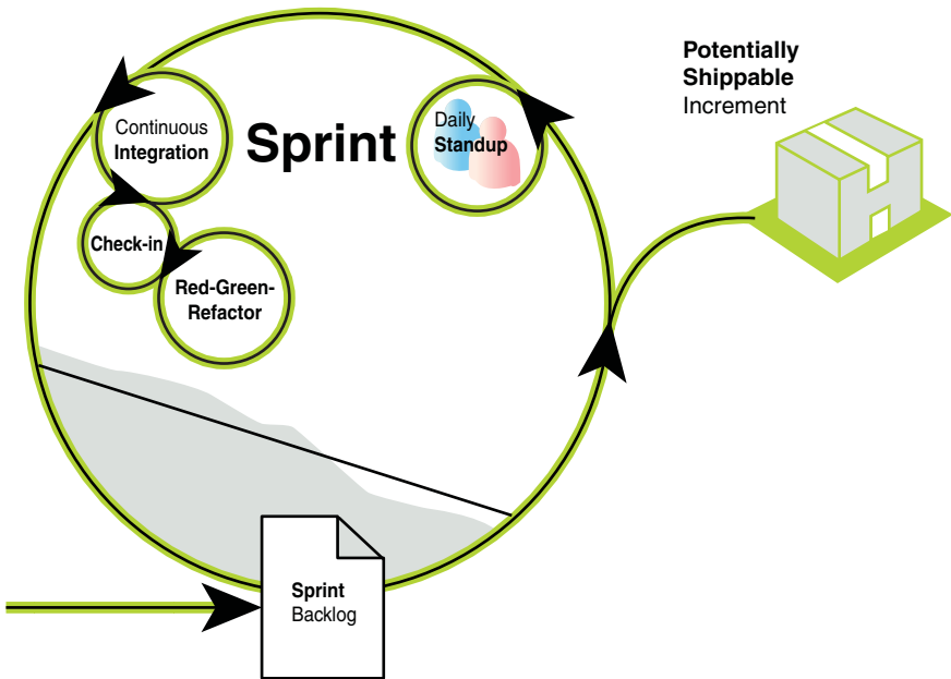
FIGURE 6-2: During a sprint, the team turns product backlog items into a potentially shippable increment. The sprint backlog contains the tasks required to achieve this, and the developers repeat the Red-Green-Refactor cycle multiple times until the code is being checked in to version control.
