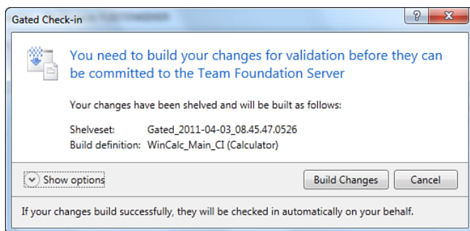
FIGURE 6-8: If gated check-in is enabled, check-ins are stored in shelvesets and validated by the build server, running all the usual build steps, before being committed to the version control repository. If the build fails, the check-in is not committed.
