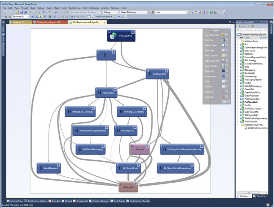
FIGURE 5-2: VS generates dependency graphs that represent all the actual references in code to understand how individual parts of the system fit together. The wider the arrows, the more references exist between two nodes.
