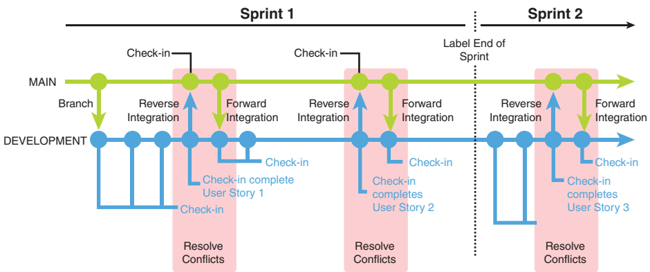
FIGURE 6-37: Branching by feature allows teams to work in parallel work streams and integrate changes once they meet a defined set of done criteria.
