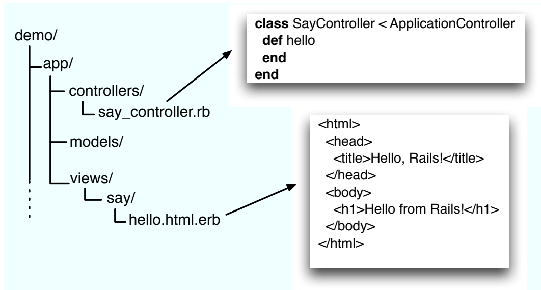
Figure 4.4: Standard Locations for Controllers and Views
