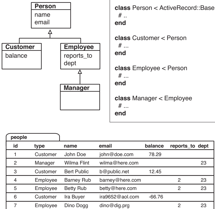
Figure 18.2: Single-Table Inheritance: A Hierarchy of Four Classes Mapped into One Table
