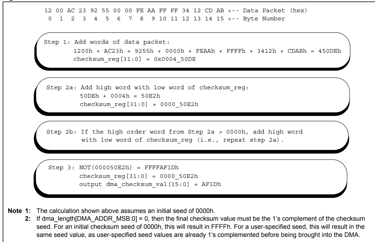
Figure 35-7: Checksum Calculation
