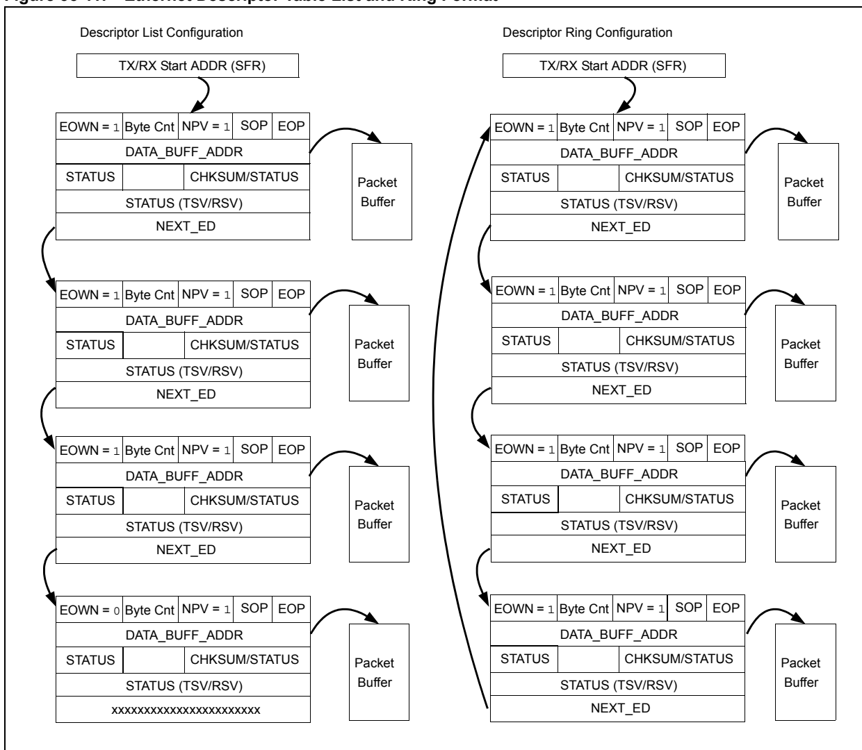
Figure 35-11: Ethernet Descriptor Table List and Ring Format
