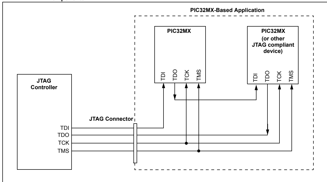
Figure 33-3: Overview of PIC32MX Family-Based JTAG Compliant Application Showing Daisy-Chaining of Components
