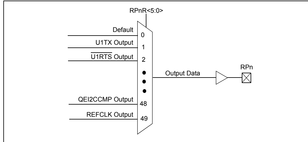
Figure 10-5: Multiplexing of Remappable Output for RPn
