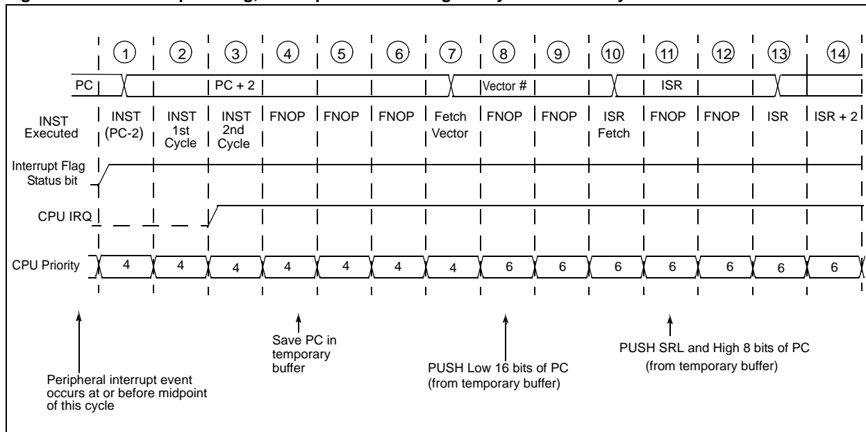
Figure 6-5: Interrupt Timing, Interrupt Occurs During 1st Cycle of a Two-Cycle Instruction
