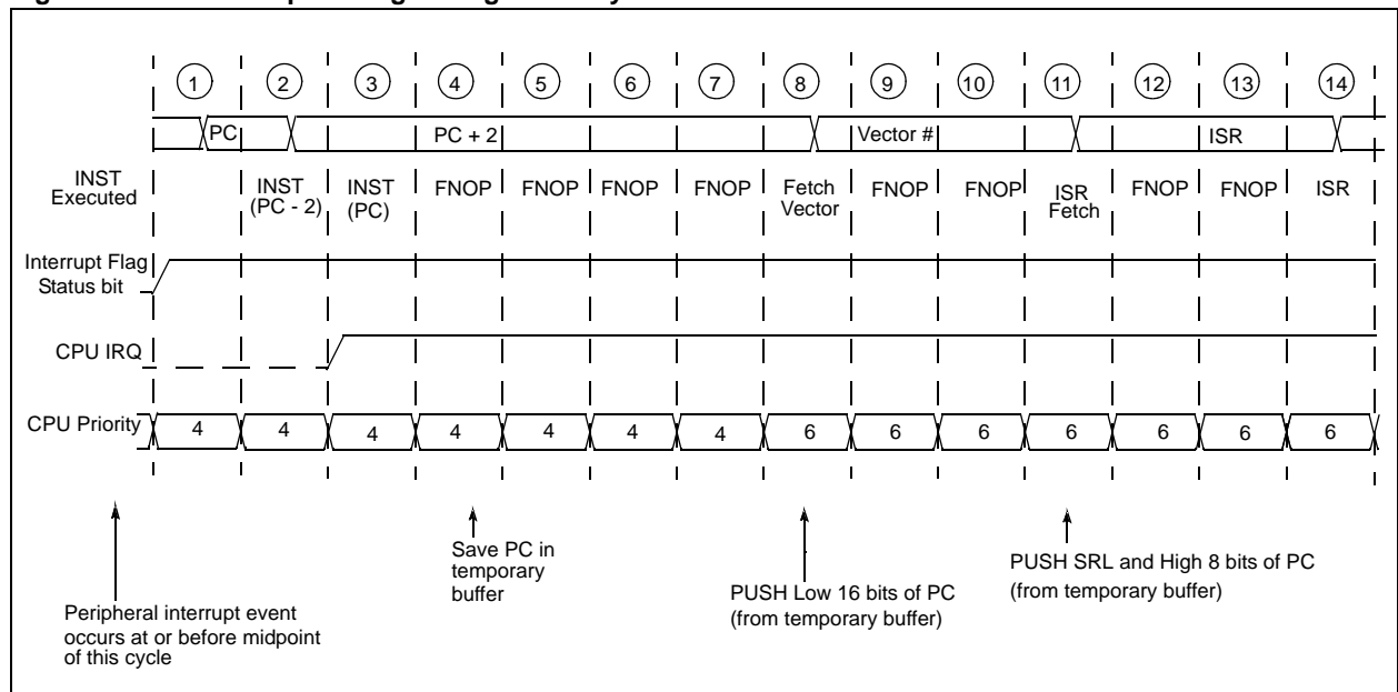
Figure 6-3: Interrupt Timing During a One-Cycle Instruction
