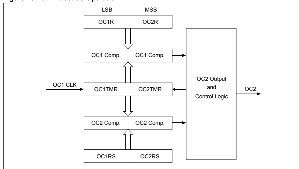
Figure 13-26: Cascade Operation
