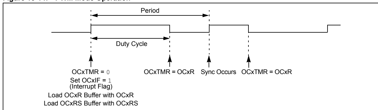
Figure 13-14: PWM Mode Operation
