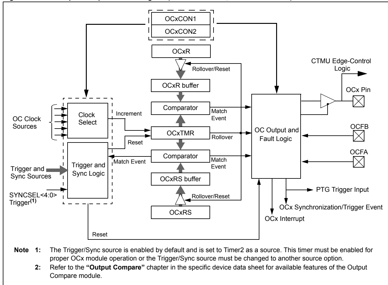
Figure 13-1: Output Compare Block Diagram (Double-Buffered, 16-bit PWM Mode)
