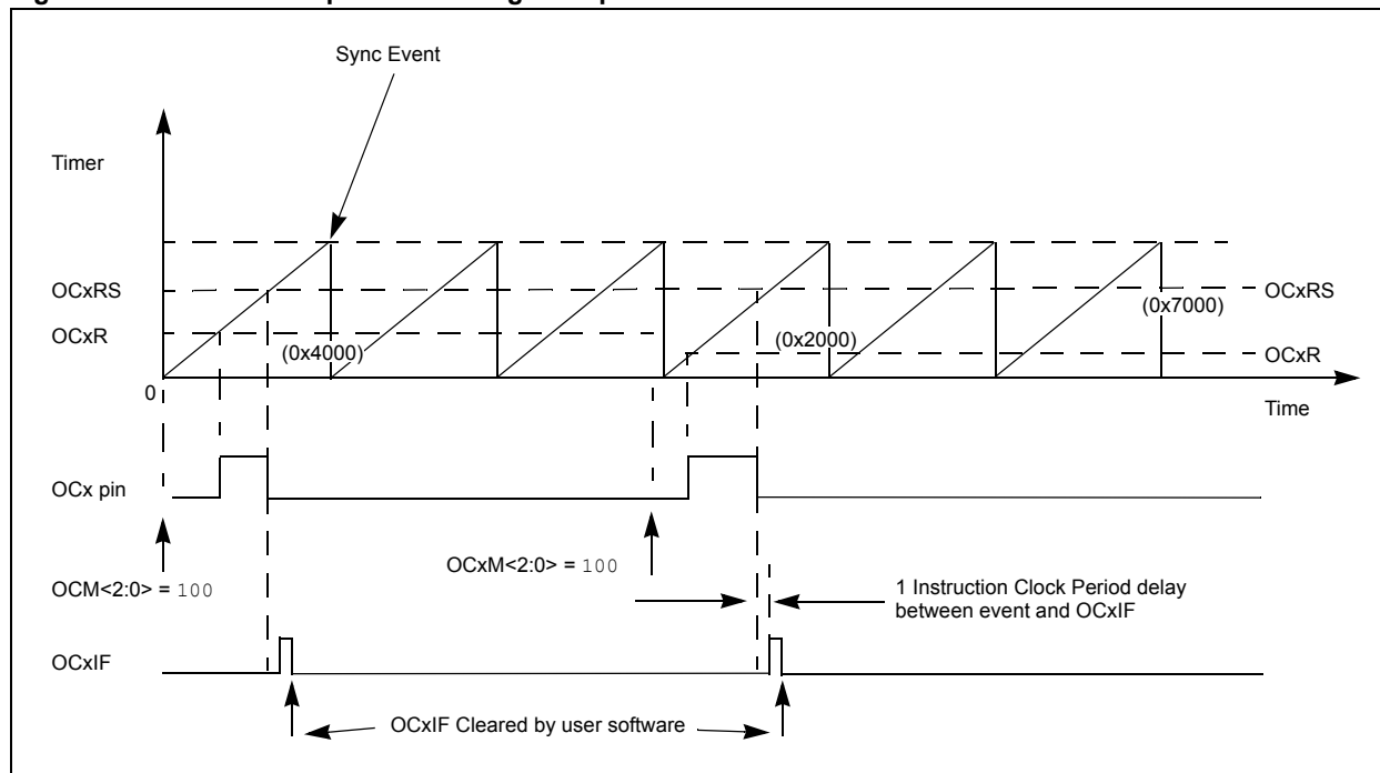
Figure 13-6: Dual Compare Mode Single Output Pulse
