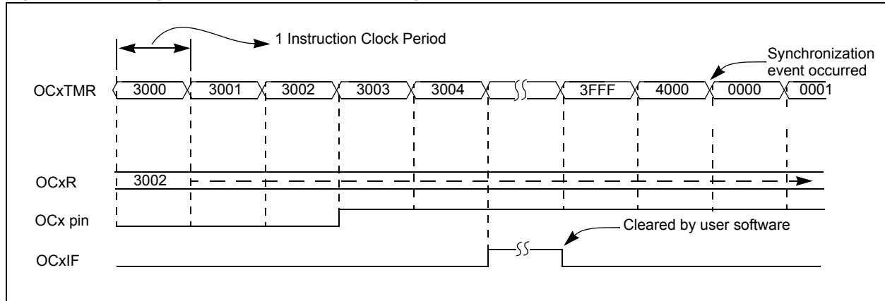
Figure 13-2: Single Compare Mode – Set OCx High on Compare Match Event
