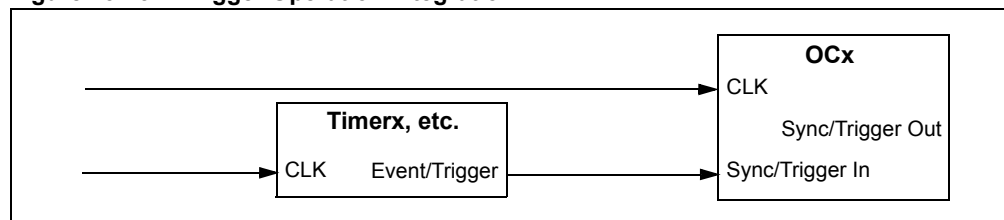
Figure 13-25: Trigger Operation Integration
