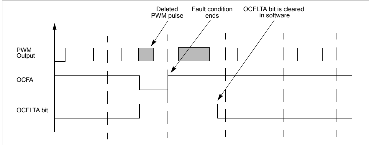
Figure 13-21: Fault Input Pin Timing, Inactive Mode (OCFA Pin Example)
