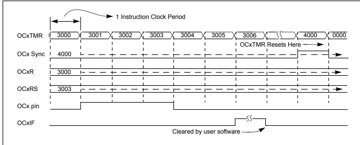
Figure 13-7: Dual Compare Mode
